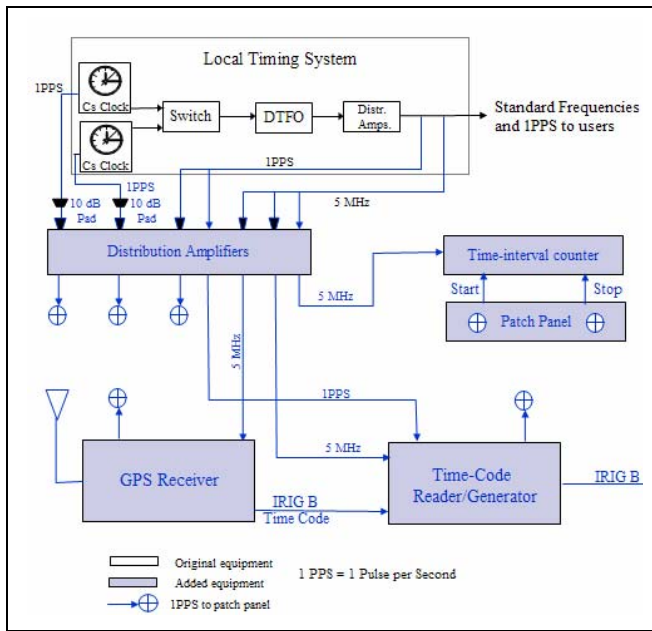
Figure 2. Equipment modifications made to the local timing system.
