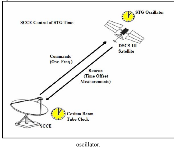
Figure 1. View of connection between local cesium clock and satellite
