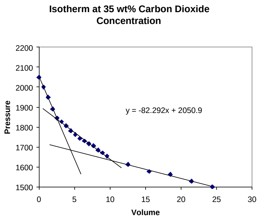
Figure 6.3.1b Pressure volume isothermo for PEG 4600 with two phase transitions
