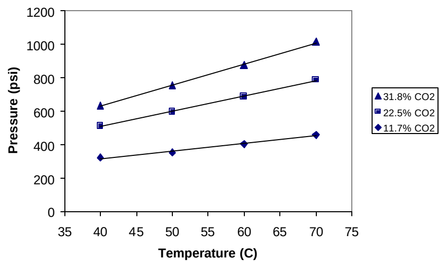
Figure 9.2: Effect of increasing solute concentration in system #2
