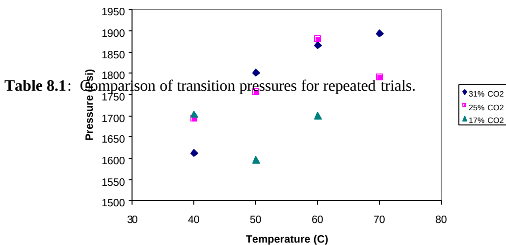
Figure 8.5. P-T plot of potential cloud points showing no clear trend.
