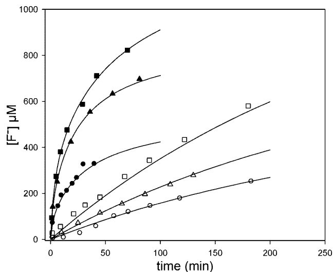
Figure 4. Time course of fluoride ions released from soman, in the presence and absence of FAF-HSA. Soman ( [S]_0 = \bullet\circ, 0.52 , \blacktriangle\blacktriangle , 0.78, \blacksquare\blacksquare , 1.3 mM) was incubated with albumin ( [E] = 0.78 mM) (filled symbols), or soman was incubated by itself through spontaneous hydrolysis (open symbols on continuous curves). Both reactions were in 60 mM Tris/HCl at pH 8.0.
