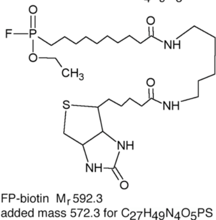
Figure 1.1. Structures of organophosphorus agents.
