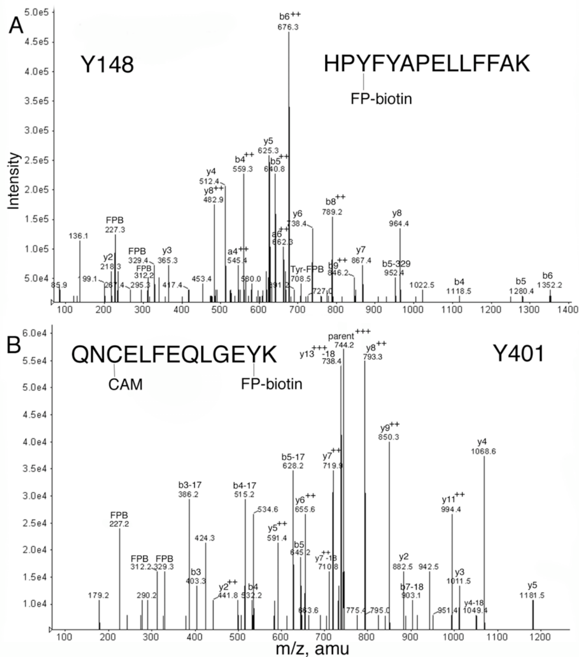
Figure 1.3. MS/MS spectra of albumin peptides labeled with FP-biotin on Tyrosine. A) Tyr 148 in peptide HPYFYAPELLFFAK, and B) Tyr 401 in peptide QNCELFEQLGEYK are covalently modified by FP-biotin. The quadruply charged parent ion in A has a mass of 579.7 m/z. The triply charged parent ion in B has a mass of 744.2 m/z.
