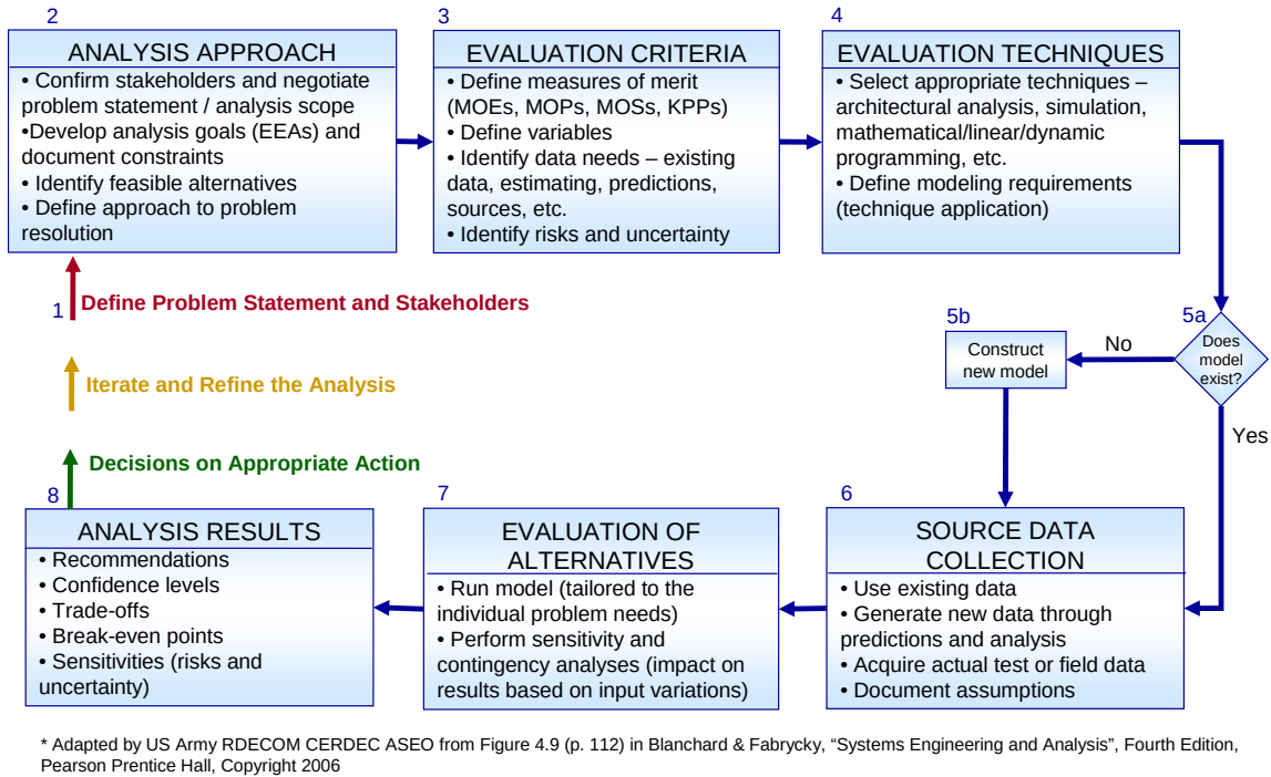
Figure 2 ASEO Systems Engineering Analysis Process
