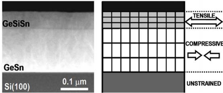
Figure 5. Left: XTEM, Z-contrast image of a tensile strained \text{Ge}_{0.64}\text{Si}_{0.32}\text{Sn}_{0.04} epilayer (light contrast) and a compressively strained \text{Ge}_{0.97}\text{Sn}_{0.03} buffer. The film surface is flat and the both layers are highly uniform and perfectly coherent. Right: schematic of the heterostructure illustrating the relative strain states of the epilayer and buffer when they share a common parallel lattice constant (see Ref. 8)
