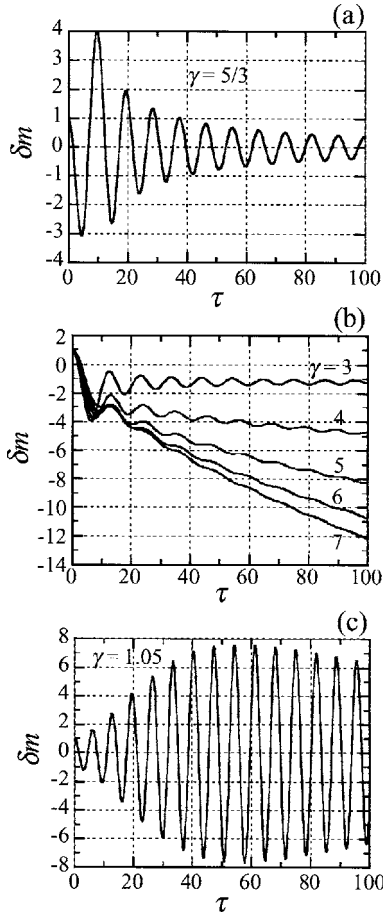
FIG. 1. Time histories of areal mass variation in a rippled expansion wave for moderate \gamma = \frac{5}{3} (a), large \gamma = 3 to 7 (b), and small \gamma = 1.05 (c).
