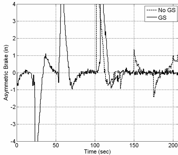
Fig. 24 Simulated Precision Placement Asymmetric Control.
