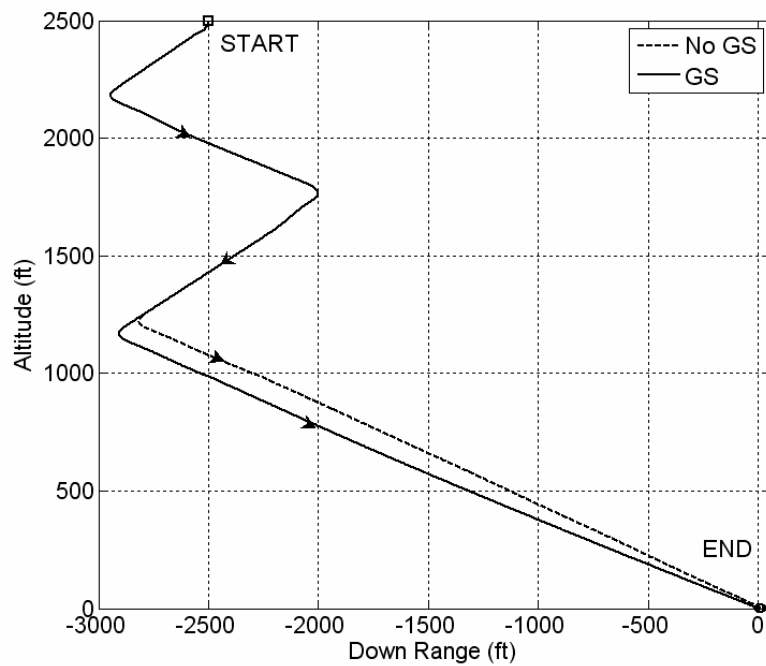
Fig. 21 Simulated Precision Placement Altitude
