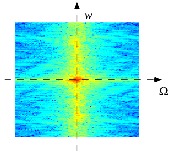
Fourier transform of the envelope of the spectrogram
