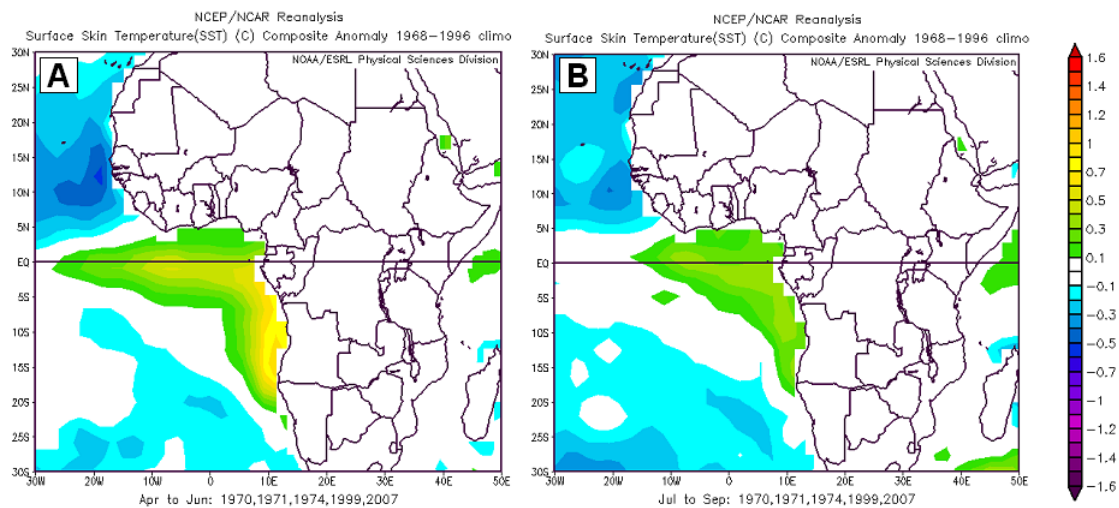
Figure 37. SST composite anomalies for +/+ | \text{LN} years for (A) AMJ, and (B) JAS. Units: ^{\circ}\text{C} .
