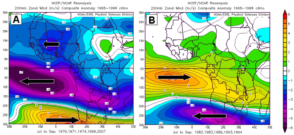
Figure 26. JAS 200 hPa zonal wind composite anomalies for: (A) +/+ | \text{LN} years; and (B) -/- | \text{EN} years. Negative (positive) anomalies indicate easterly (westerly) anomalies. Black arrows show anomalous wind directions. Units: \text{m s}^{-1} .
