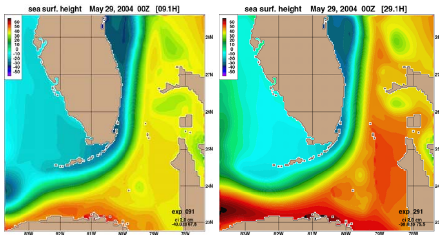
Figure 1. SoFLA domain sea surface height (SSH) on 5/29/04 from twin experiments with initial and boundary conditions from the HYCOM-FREE (left) and HYCOM-NCODA Gulf of Mexico simulations (right).
