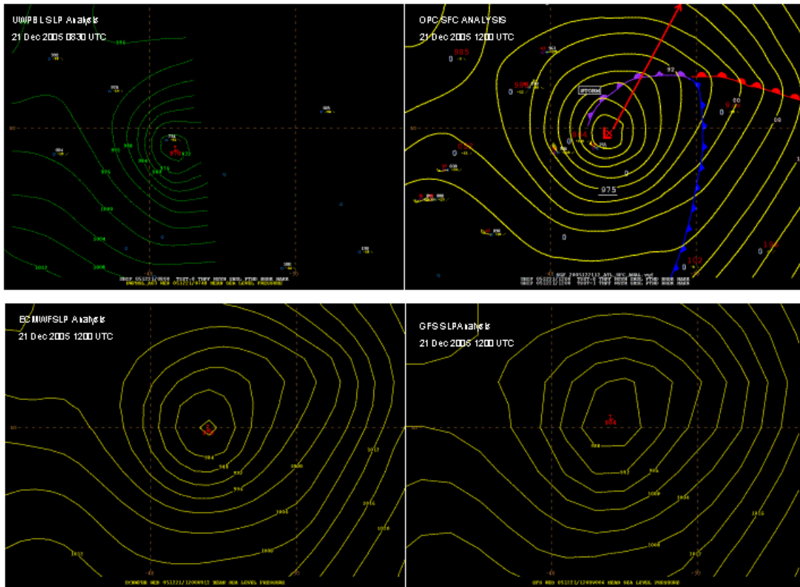
Figure 4. Four panel showing the UW PBL sea level pressure field from 21 Dec 2005 (upper left), OPC surface analysis for 1200 UTC 21 Dec 2005 (upper right), 12 hour forecast from the 00 UTC 21 Dec 2005 ECMWF run (lower left), and 06 hour forecast from the NCEP GFS valid 1200 UTC 21 Dec 2005.
