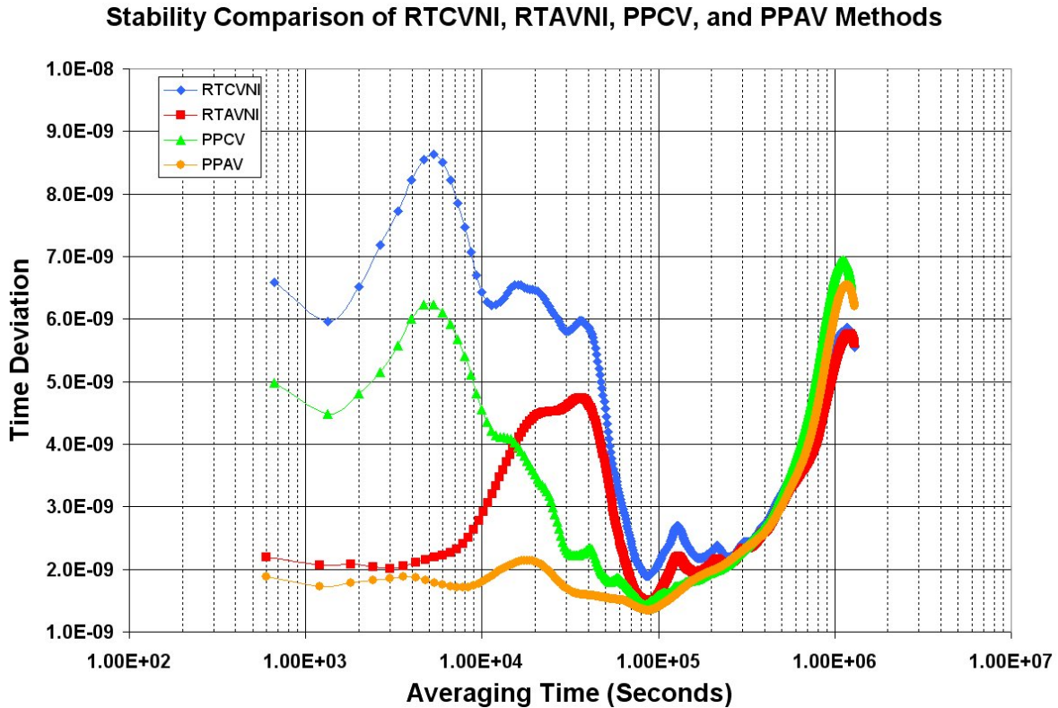
Figure 7. TDEV graph comparing the RTCVNI, RTAVNI, PPCV, and PPAV methods.
