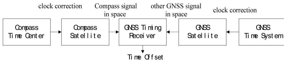
Figure 1. Determination via a multi-mode GNSS timing receiver.
