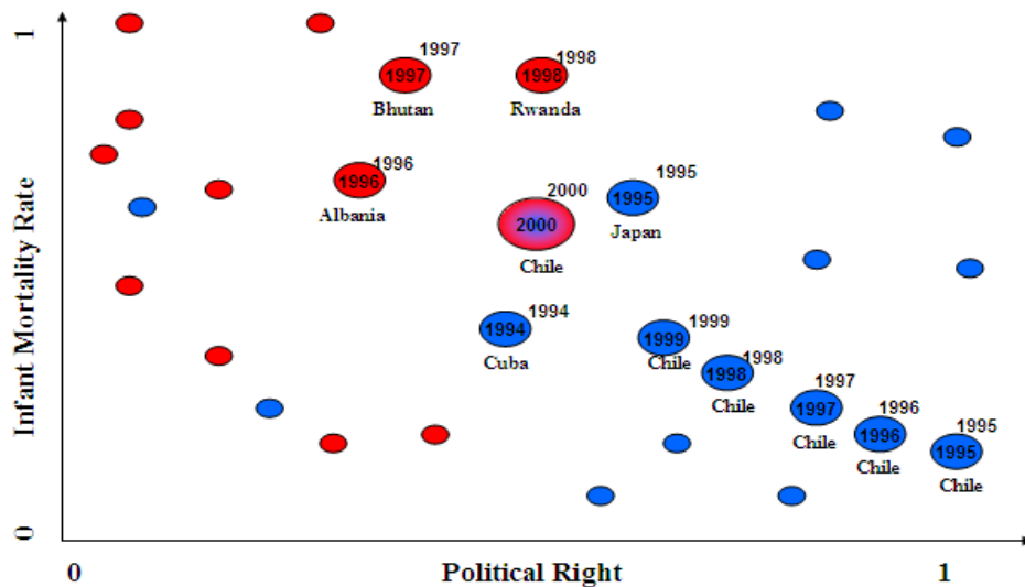
Figure 4. Prediction from the raw data set. The two feature variables (Political Right and Infant Mortality Rate) had been scaled between 0 and 1.
