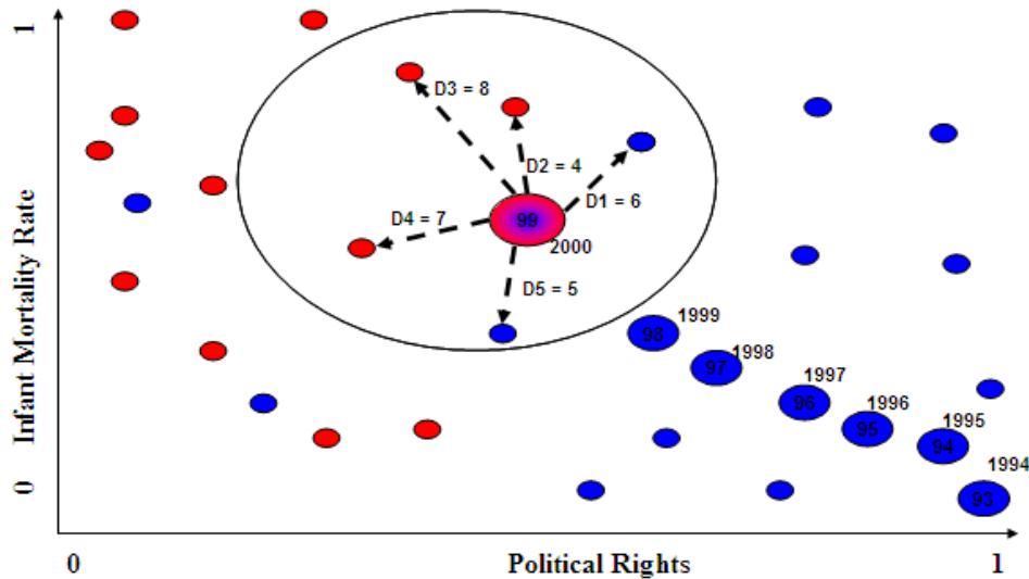
Figure 9. Predict conflict potential by the closest neighbors weighted by the inverse of distance. D# refers to the distance between point # and the predicted point.
