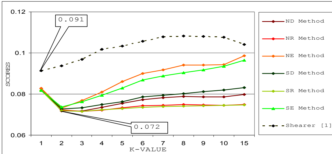
Figure 12. Result: Two-Year-Out Prediction (1998-2003). The best predicted result is give by ND method at k =2. This method improves by 0.019 from the Shearer method.
