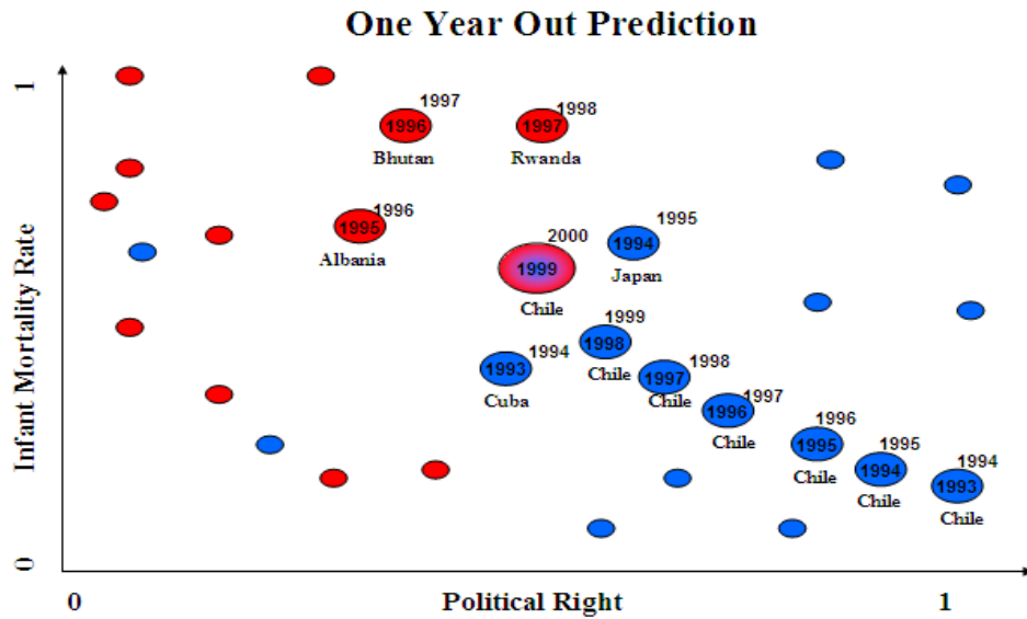
Figure 5. One-Year-Out-Prediction. The points are painted with the color based on the conflict-peace status from one year later.
