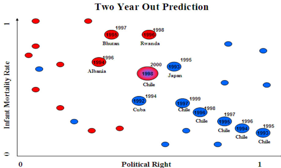
Figure 6. Two-Year-Out-Prediction. The points are painted with the color based on the conflict-peace status from two years later.
