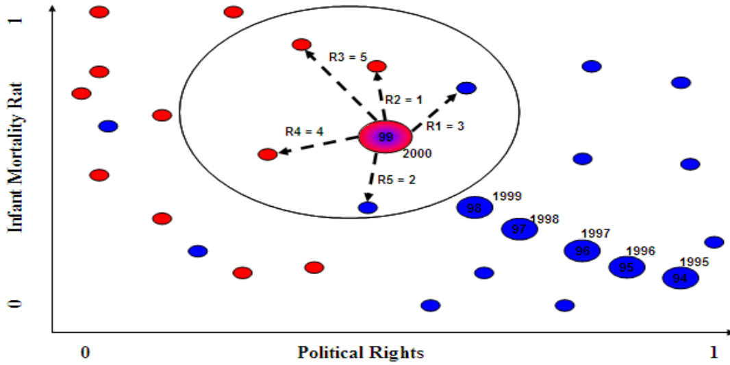
Figure 10. Predict conflict potential by the closest neighbors weighted by the inverse of rank. R_{\#} refers to the rank between point # and the predicted point.
