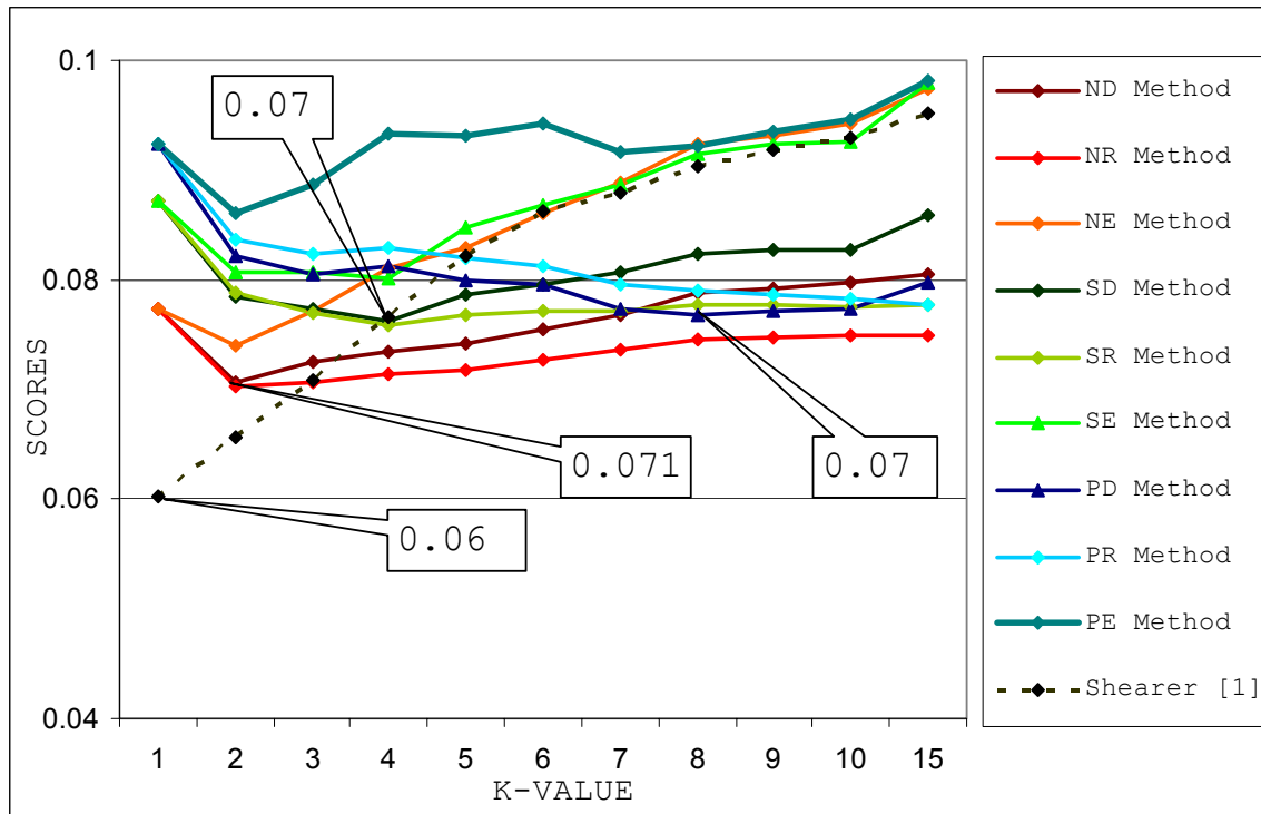
Figure 11. Result: One-Year-Out Prediction (1998-2003). The lowest score of all methods is given by the Shearer method. The lowest score of this study's proposed methods is given by ND method. The difference is 0.011.
