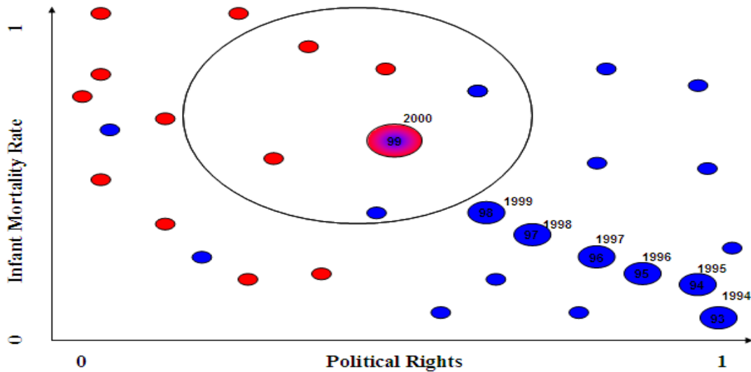
Figure 8. Predict conflict potential by equally weighting the closest neighbors.
