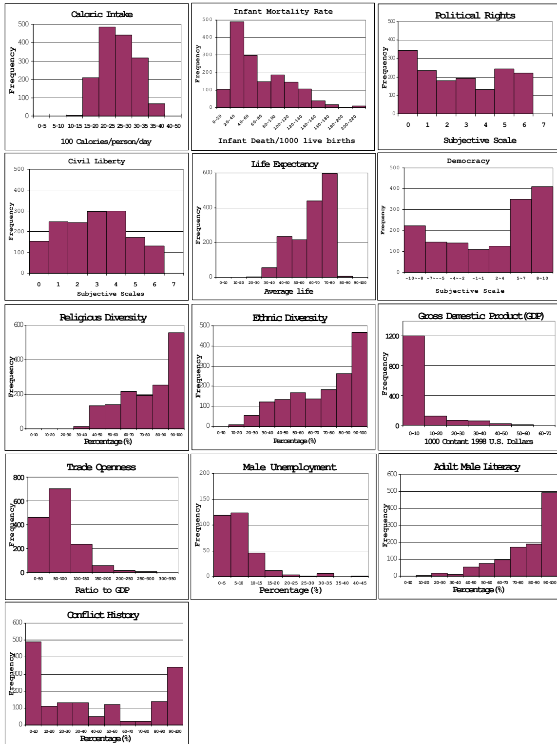
Figure 1. Variable Distribution.
