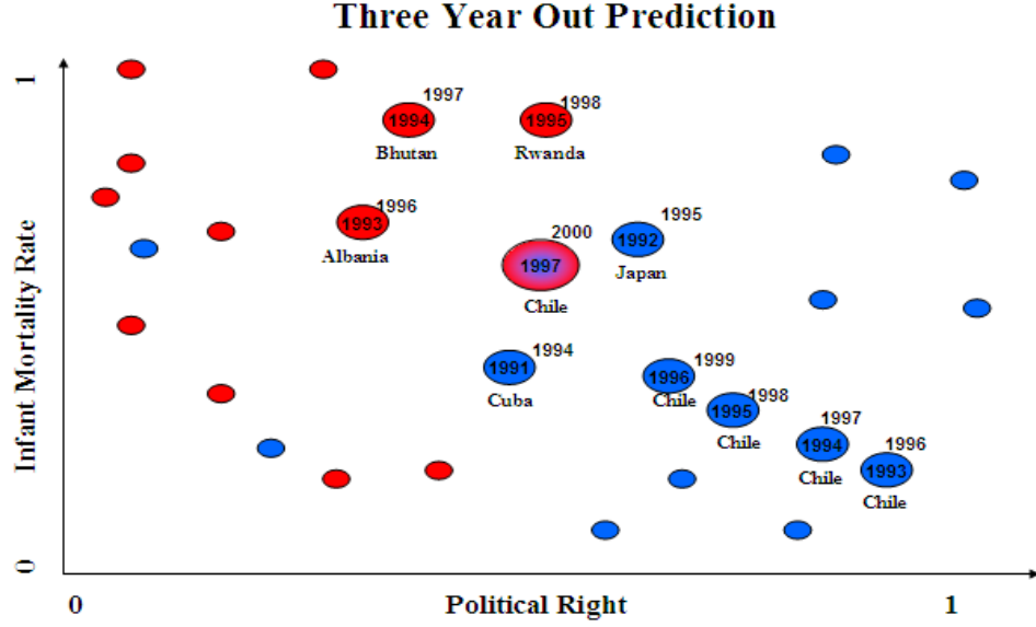
Figure 7. Three-Year-Out-Prediction. The points are painted with the color based on the conflict-peace status from three years later.
