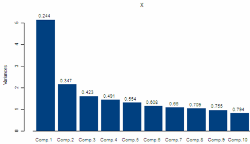
Figure 2. Scree Plot of principal components. Each number on the top of bar in the plot indicates the proportion of variance. Here, there are only 10 components to view, but this plot gives the same information as the important components indicated above.
