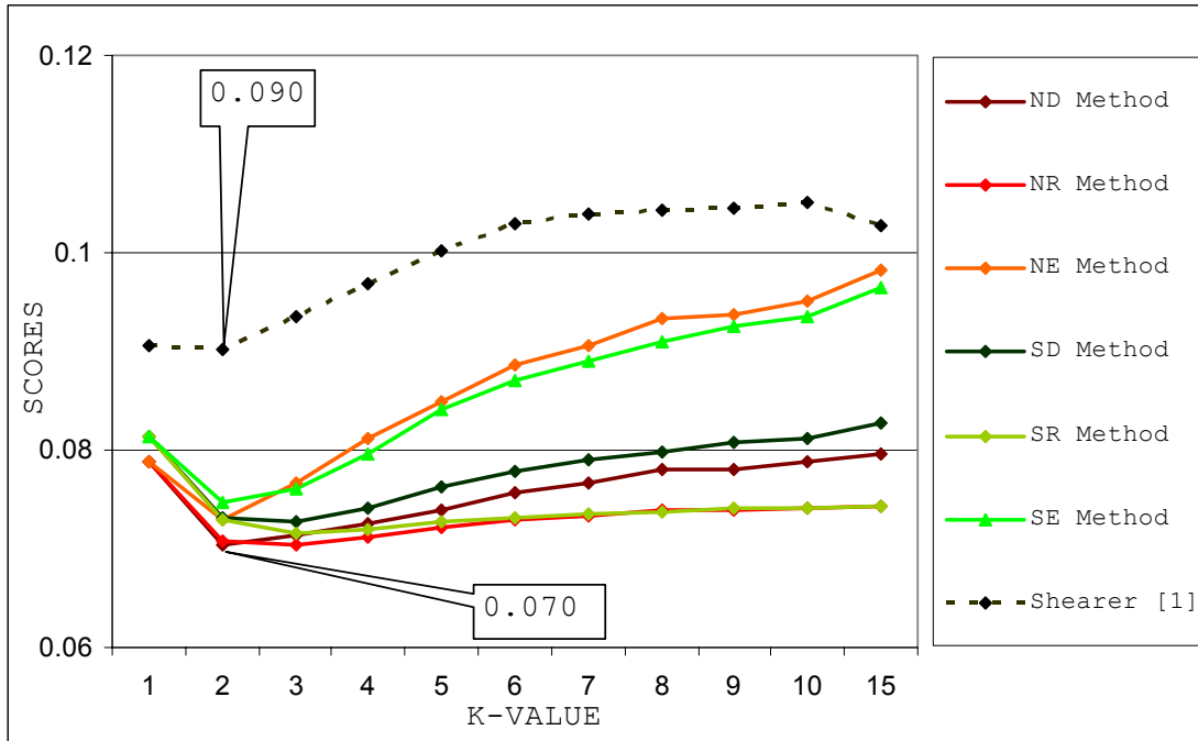
Figure 14. Result: Overall Prediction (1993-2003). The best predicted result is given by ND method at k=2 . This method improves by 0.019 from the Shearer method.
