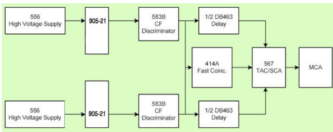
Figure 11. Fast-fast PALS.(11)
