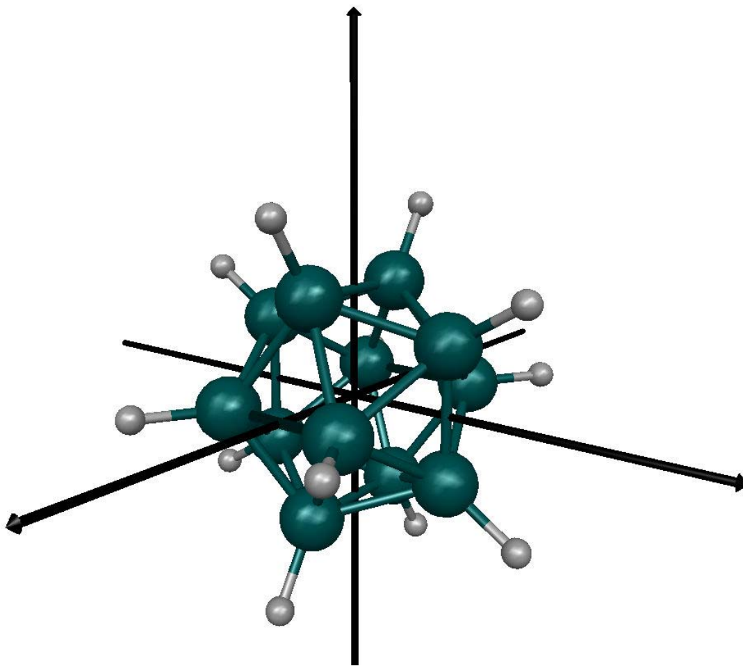
Figure 7. B_{12}H_{12} geometry.
