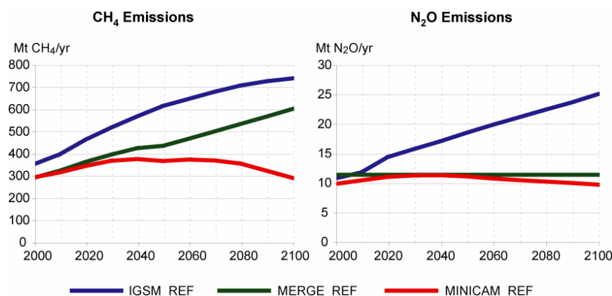
Figure IV.15. Projected global CH 4 and N 2 O emissions across three CCSP reference scenarios. Global anthropogenic emissions of CH 4 and N 2 O vary widely among the reference scenarios. There is uncertainty in year-2000 CH 4 emissions, with MIT's IGSM reference scenario ascribing more of the emissions to human activity and less to natural sources. Differences in scenarios reflect, to a large extent, different assumptions about whether current emissions rates will be reduced significantly for other reasons, for example, whether higher natural gas prices will stimulate capture of CH 4 for use as a fuel. Source: Clarke et al. (2007).
