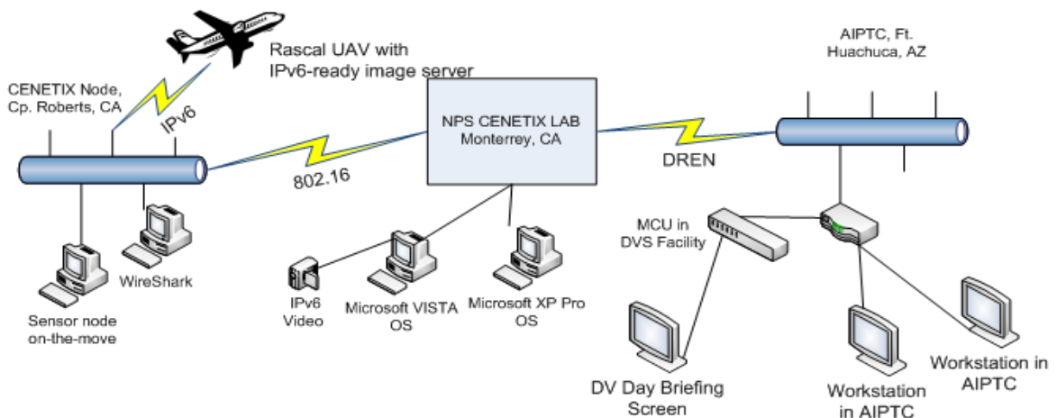
Figure 14. TNT Architecture IPv6 TNT 08-03
