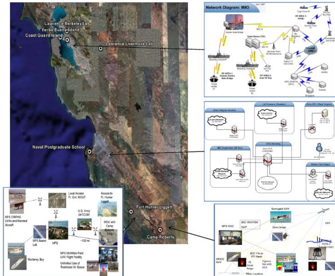
Figure 7. Diagram of CENETIX Network (After: Bordetsky and Clement, CENETIX LAB 2007)
