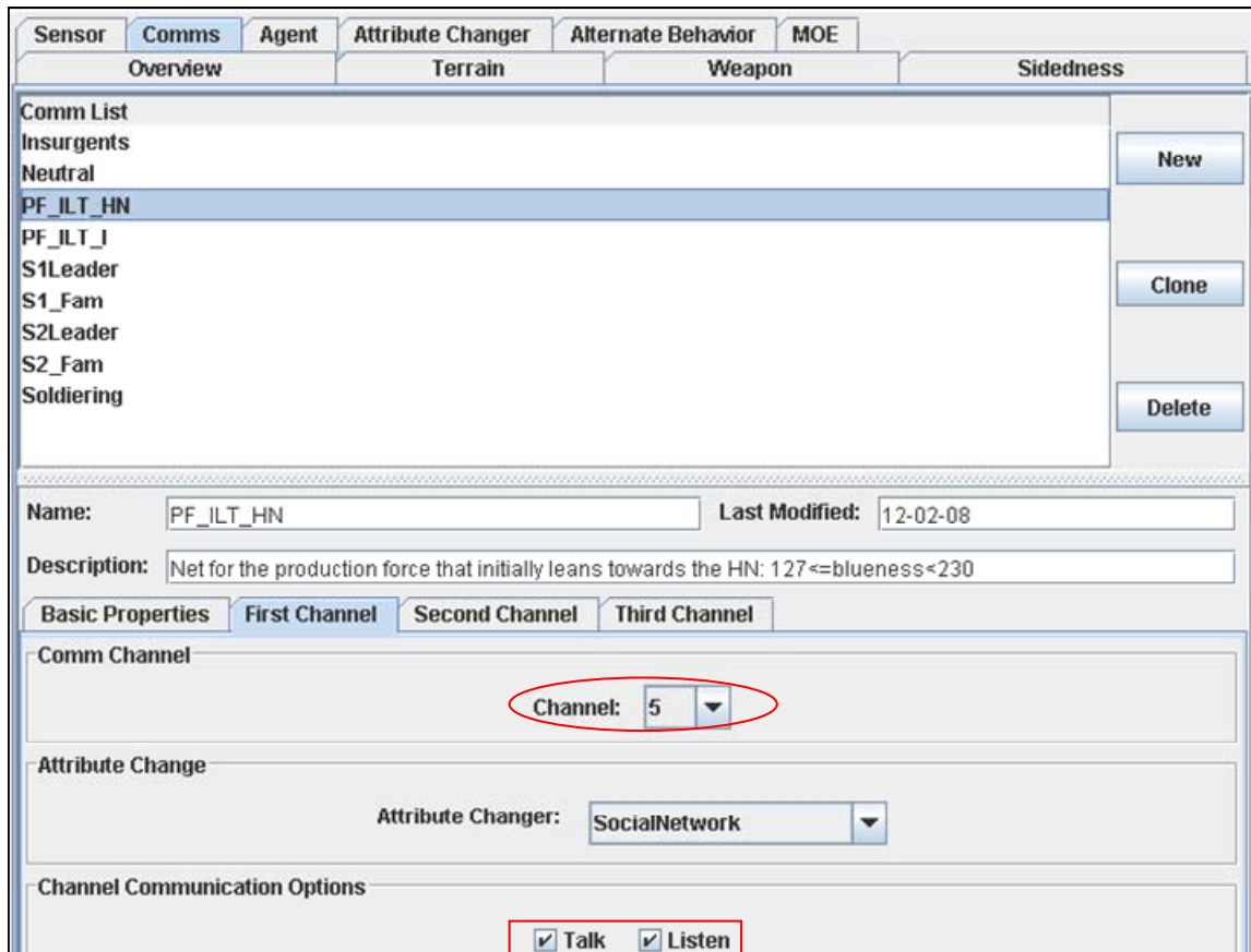
Figure 11. Channel and functionality designation for PF_ILT_HN network (from Pythagoras 2.0.0 Version 19).
