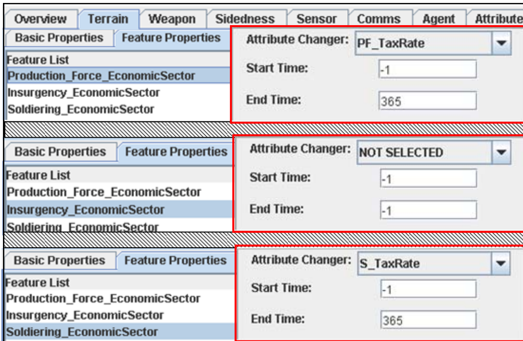
Figure 23. Tax rate implementation for the three sectors of the economy (from Pythagoras 2.0.0 Version 19).
