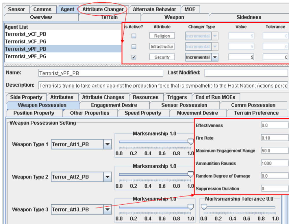
Figure 8. Terrorist_vPF_PB actor agent setup for permanent influence implementation (from Pythagoras 2.0.0 Version 19).
