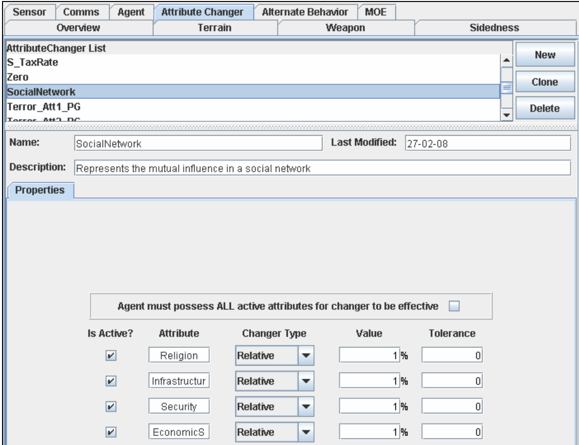
Figure 13. “SocialNetwork” attribute changer implementation (from Pythagoras 2.0.0 Version 19).
