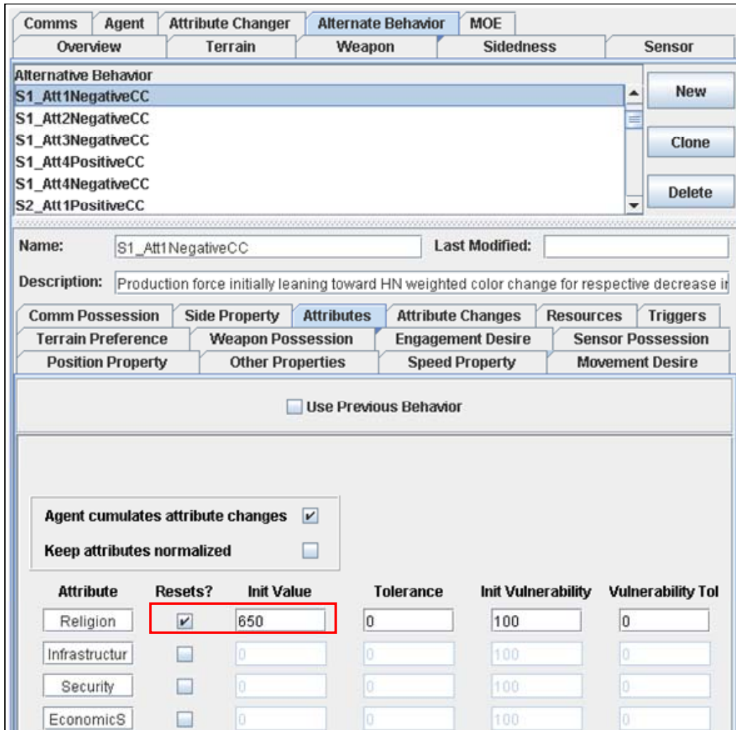
Figure 18. Resetting tripped attributes to prevent infinite triggering upon return to “Initial” (from Pythagoras 2.0.0 Version 19).
