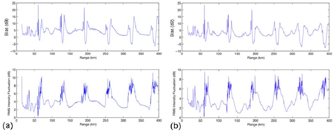
Figure 26. (a) \Phi_b(r) and \Phi_{RMS}(r) , using Stammer spectrum, frequency 250 Hz, source depth 50m, receiver depth 50m. Statistics for run #5 show \Phi_b=5.33 dB and \Phi_{RMS}=6.18 dB. (b) As in (a), but with Lorentzian spectrum. Statistics for run #7 show \Phi_b=4.37 dB and \Phi_{RMS}=5.50 dB.
