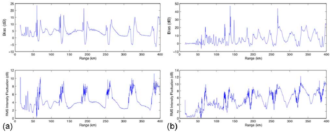
Figure 29. (a) \Phi_b(r) and \Phi_{RMS}(r) , using Stammer spectrum, frequency 250 Hz, source depth 50m, receiver depth 50m. Statistics for run #5 show \Phi_b=5.33\text{dB} and \Phi_{RMS}=6.18\text{dB} . (b) As in (a), but with source depth 200m. Statistics for run #6 show \Phi_b=5.69\text{dB} and \Phi_{RMS}=6.58\text{dB} .
