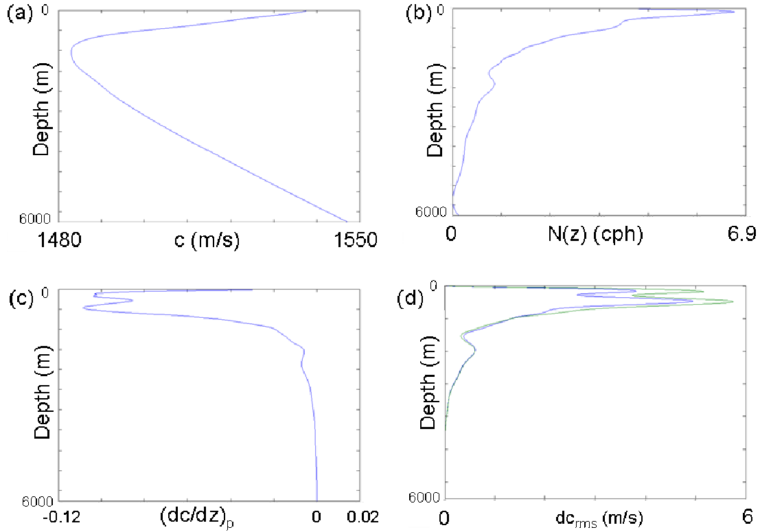
Figure 6. The background ocean profiles used in this study: (a) sound speed, (b) buoyancy frequency, (c) potential sound speed gradient, (d) RMS sound speed variability. The profiles were derived from the World Ocean Atlas 2001 annual database for 23^\circ\text{N } 125^\circ\text{E} . In (d), the blue line is the average of 32 random realization of the ocean, while the green line is the theoretical profile for the acoustic model.
