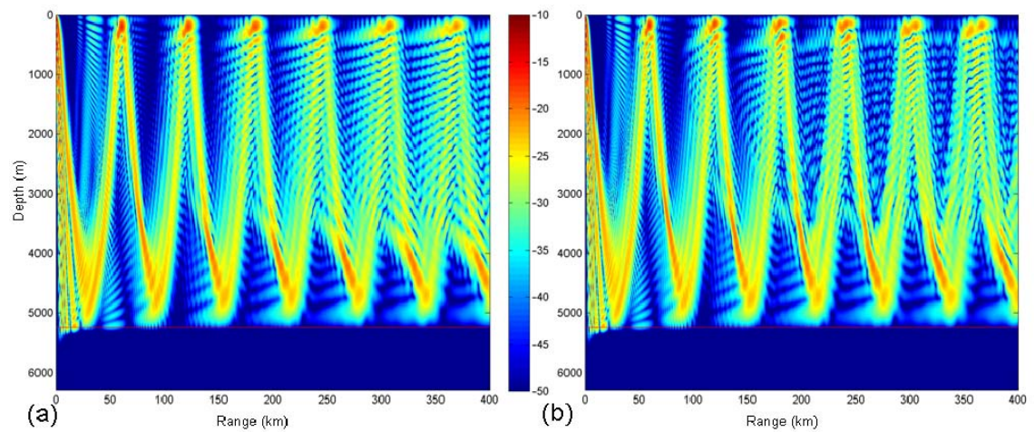
Figure 12. (a) Full water-column transmission loss diagram for unperturbed ocean: frequency 20 Hz, source depth 200m. (b) As in (a), but with ocean perturbed by Stammer eddy field. In (b), the eddy field causes spreading and shifting of the CZs.
