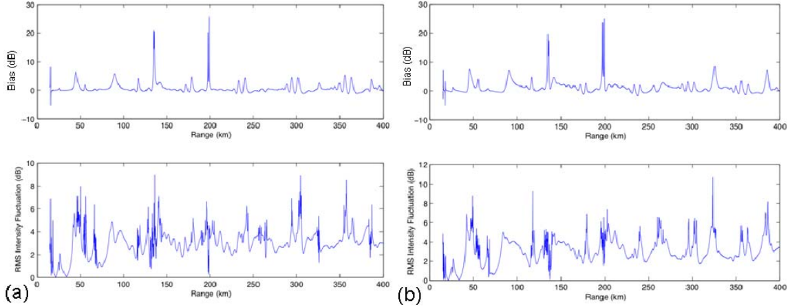
Figure 25. (a) \Phi_b(r) and \Phi_{RMS}(r) , using Stammer spectrum, frequency 20 Hz, source depth 200m, receiver depth 50m. Statistics for run #2 show \Phi_b=0.80 dB and \Phi_{RMS}=3.33 dB. (b) As in (a), but with Lorentzian spectrum. Statistics for run #4 show \Phi_b=0.88 dB and \Phi_{RMS}=3.02 dB.
