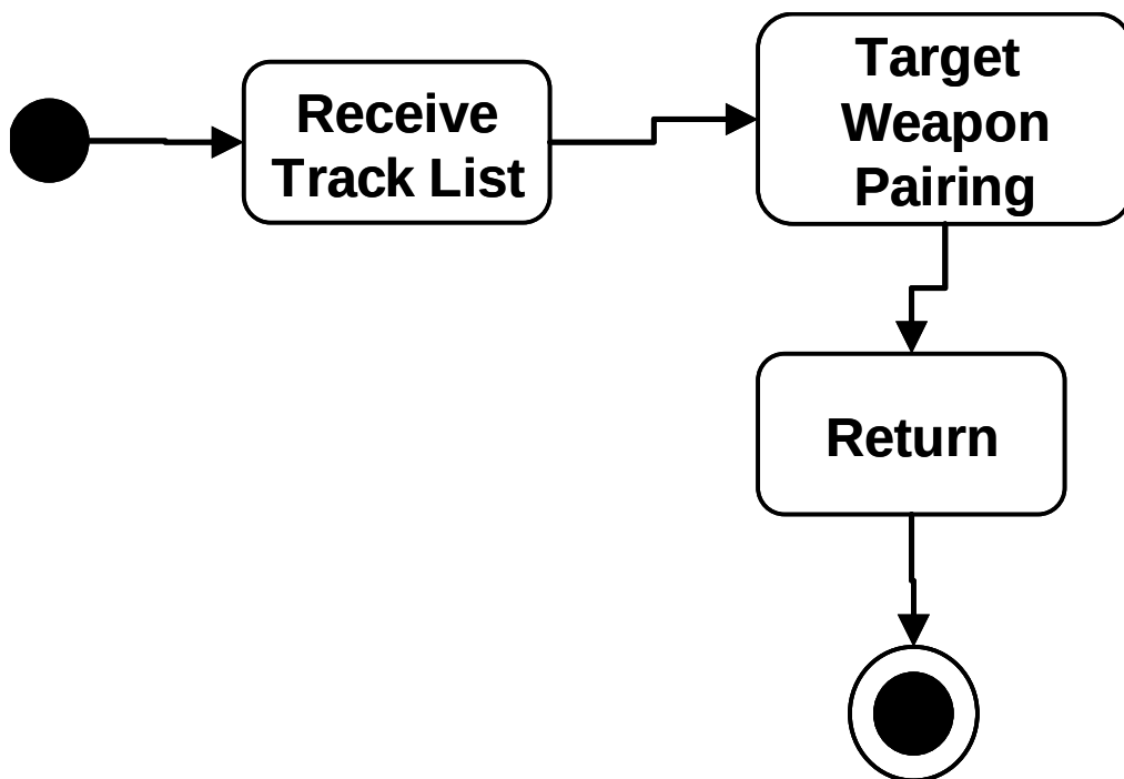
Figure 20. Assign Weapon
