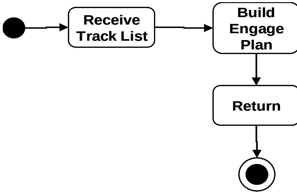
Figure 21. Engage
