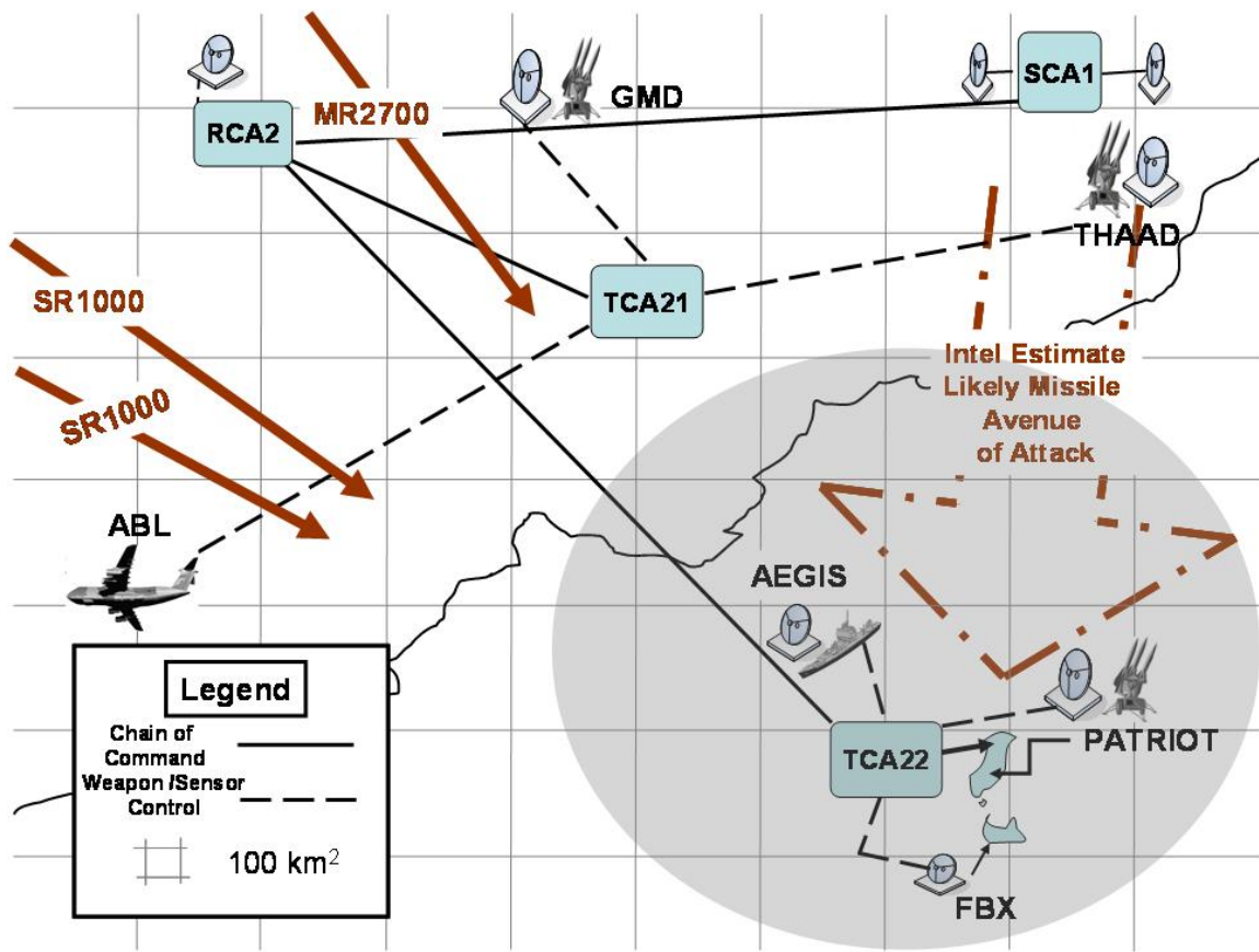
Figure 17. BMDS Scenario
