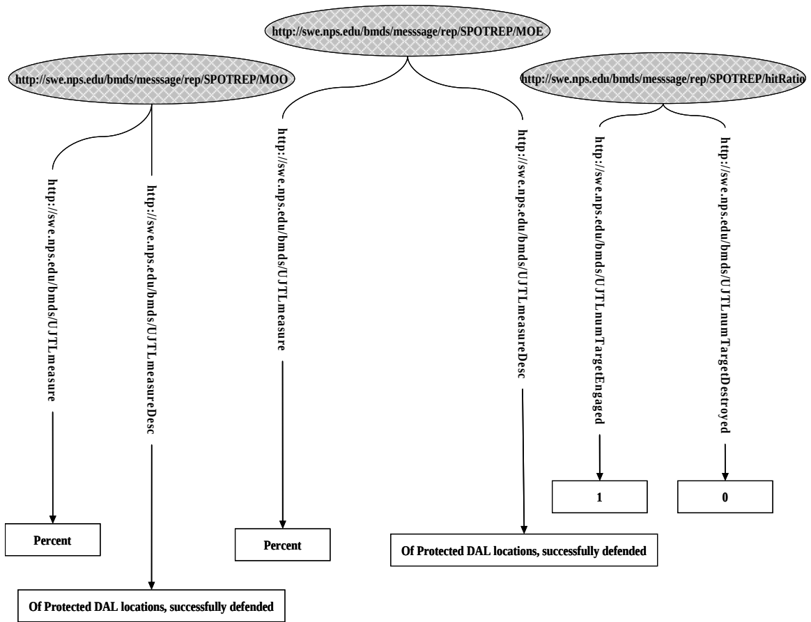
Figure 31. SPOTREP RDF Graph MOO, MOE, Hit_Ratio
