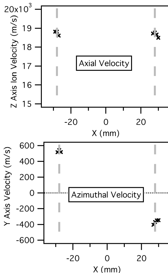
Figure 11. Axial and azimuthal velocities at X = \pm 27, \dots \pm 30 mm, Y = 0 , Z = 5 mm.
