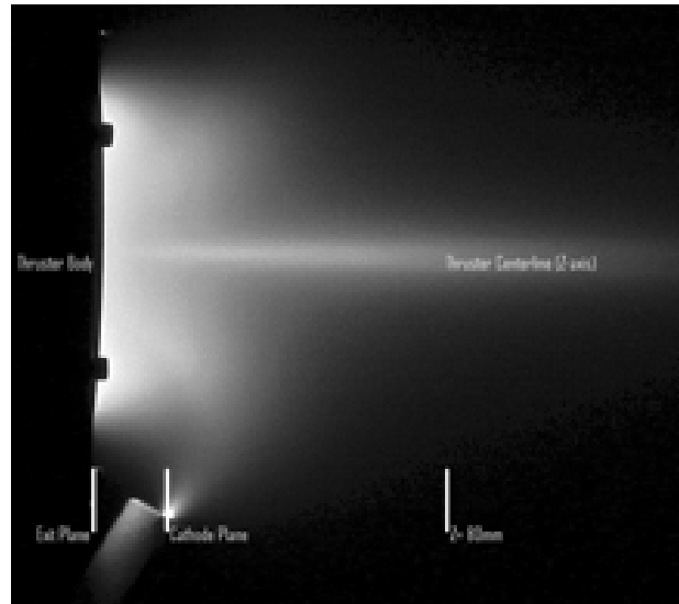
Figure 13. Photograph of the cylindrical BHT-600 Hall thruster plume with the plume central core clearly identifiable.
