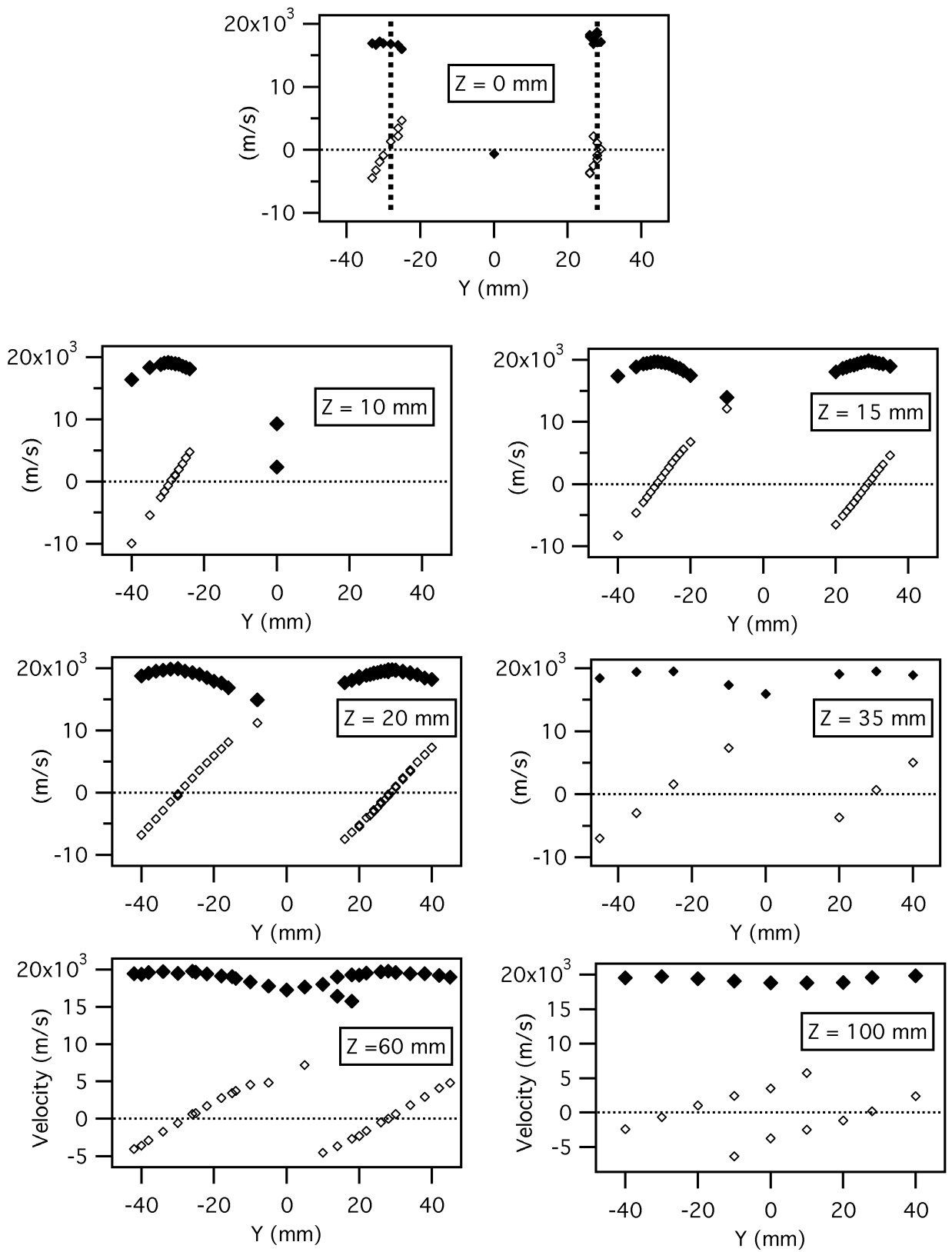
Figure 6. Ion velocity components for various locations in Z on the Y-Z plane. The closed symbols represent axial (Z) velocity components and the open symbols represent the radial (Y) velocity components.
