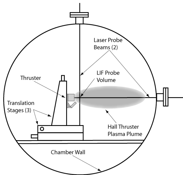
Figure 2. Side view diagram of thruster within AFRL chamber 6 showing the translation stages two and laser probe beams.
