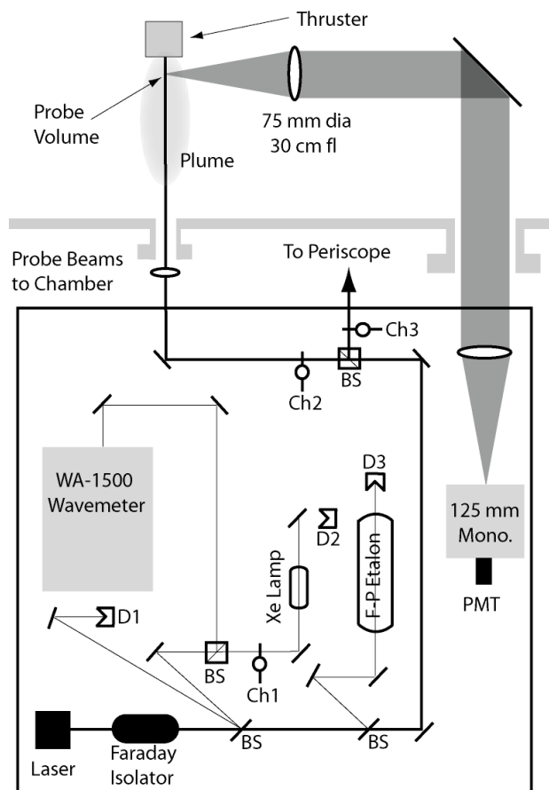
Figure 3. Top view diagram of the laser optical train and collection optics.
