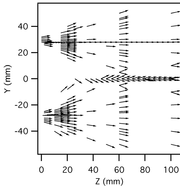
Figure 5. Ion velocity vector plot in the Y-Z plane ( X = 0 ).
