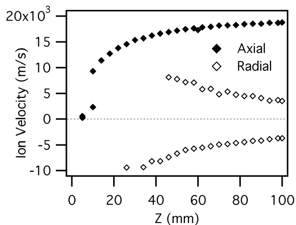
Figure 8. Acceleration channel center axial (Z) and radial (Y) on velocity components at X = Y = 0 mm.
