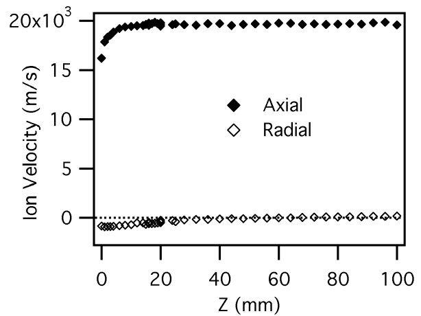
Figure 7. Acceleration channel center axial ( Z ) and radial ( Y ) on velocity components at Y = 28 mm, X = 0 .
