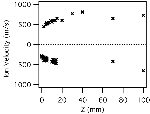
Figure 12. Azimuthal velocity evolution in to the plume ( X = \pm 27, \dots \pm 30 mm, Y = 0 , Z = 0 mm to 100 mm).
