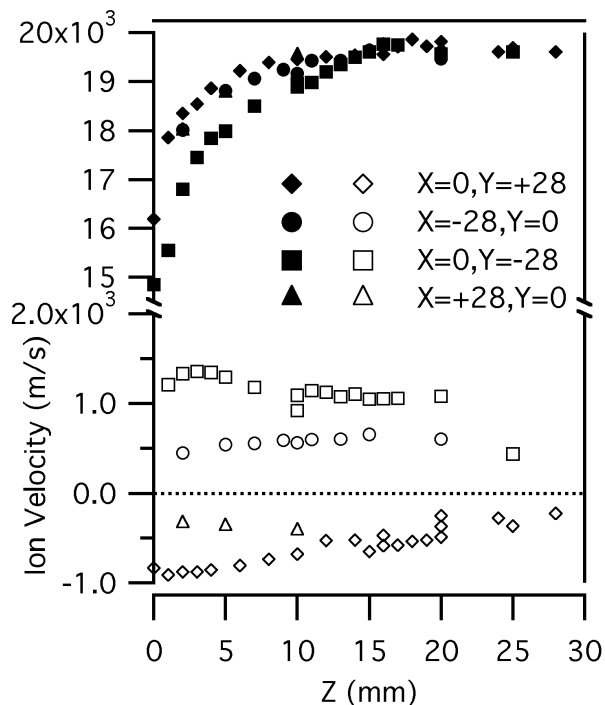
Figure 10. Z axis and Y axis ion velocity profiles for channel center ( R = 28 mm where X^2 + Y^2 = R^2 ) at the four coordinate cardinal directions. Note the solid symbols denote the Z velocity component and the open symbols the Y velocity component.
