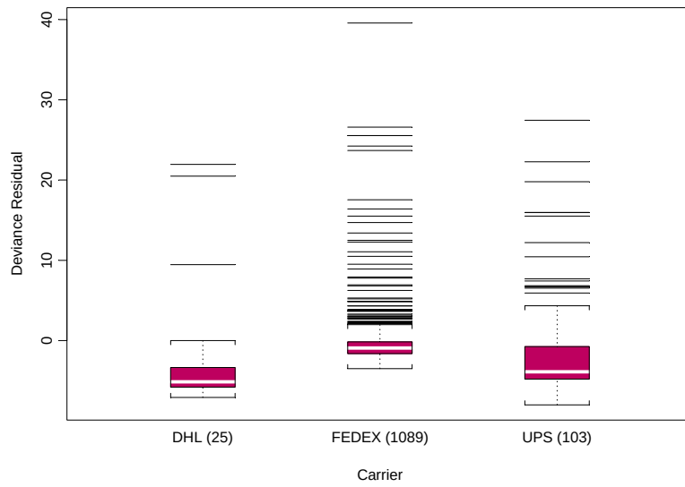
Figure L.3. Boxplot of Carrier Residual Deviances (NORFOLK)
