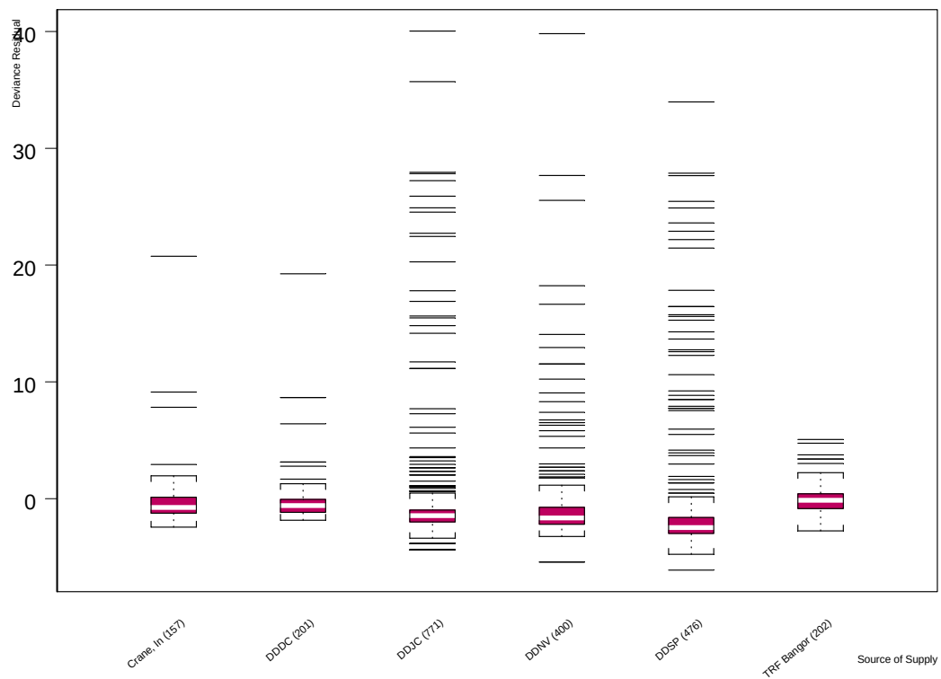
Figure N.3. Boxplot of Source of Supply Residual Deviances (PEARL HARBOR)
