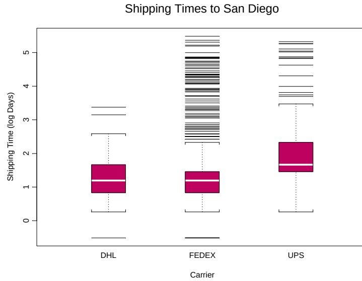
Figure P.1. Boxplot of Primary Carrier Shipping Times (SAN DIEGO)
