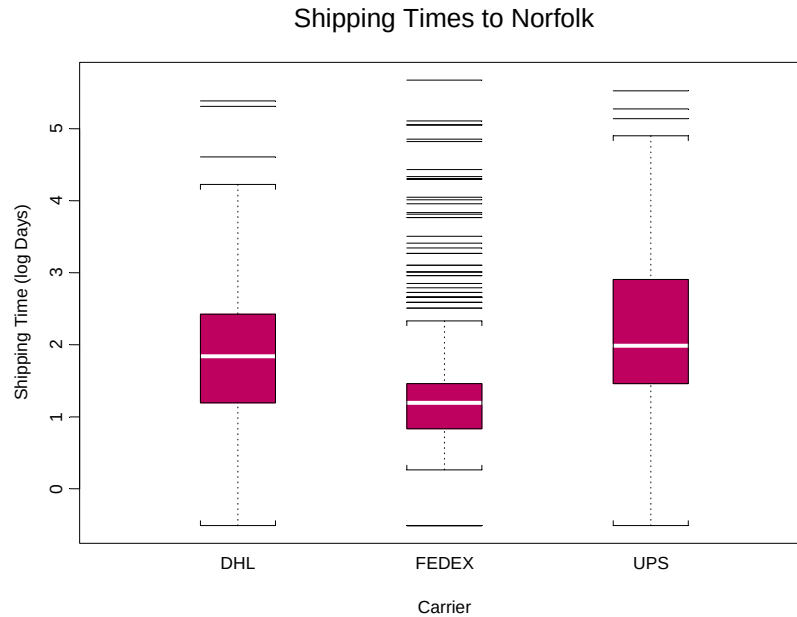
Figure L.1. Boxplot of primary Carrier Shipping Times (NORFOLK)
