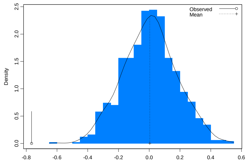
Figure 4.7. Permutation Test for Regression of Processing Time (DDPH)
