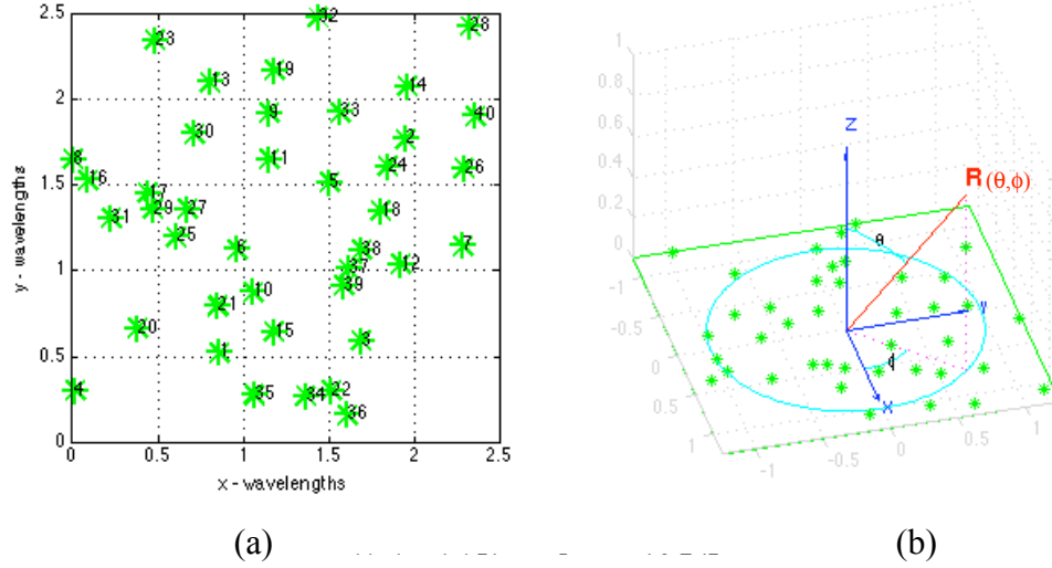
Figure 17. Searching WSN: (a) Realization of a 40 Element, 2.5\lambda \times 2.5\lambda Random Planar Array (b) Coordinate System with Scan Plane at \theta = 90^\circ Shown in Cyan
