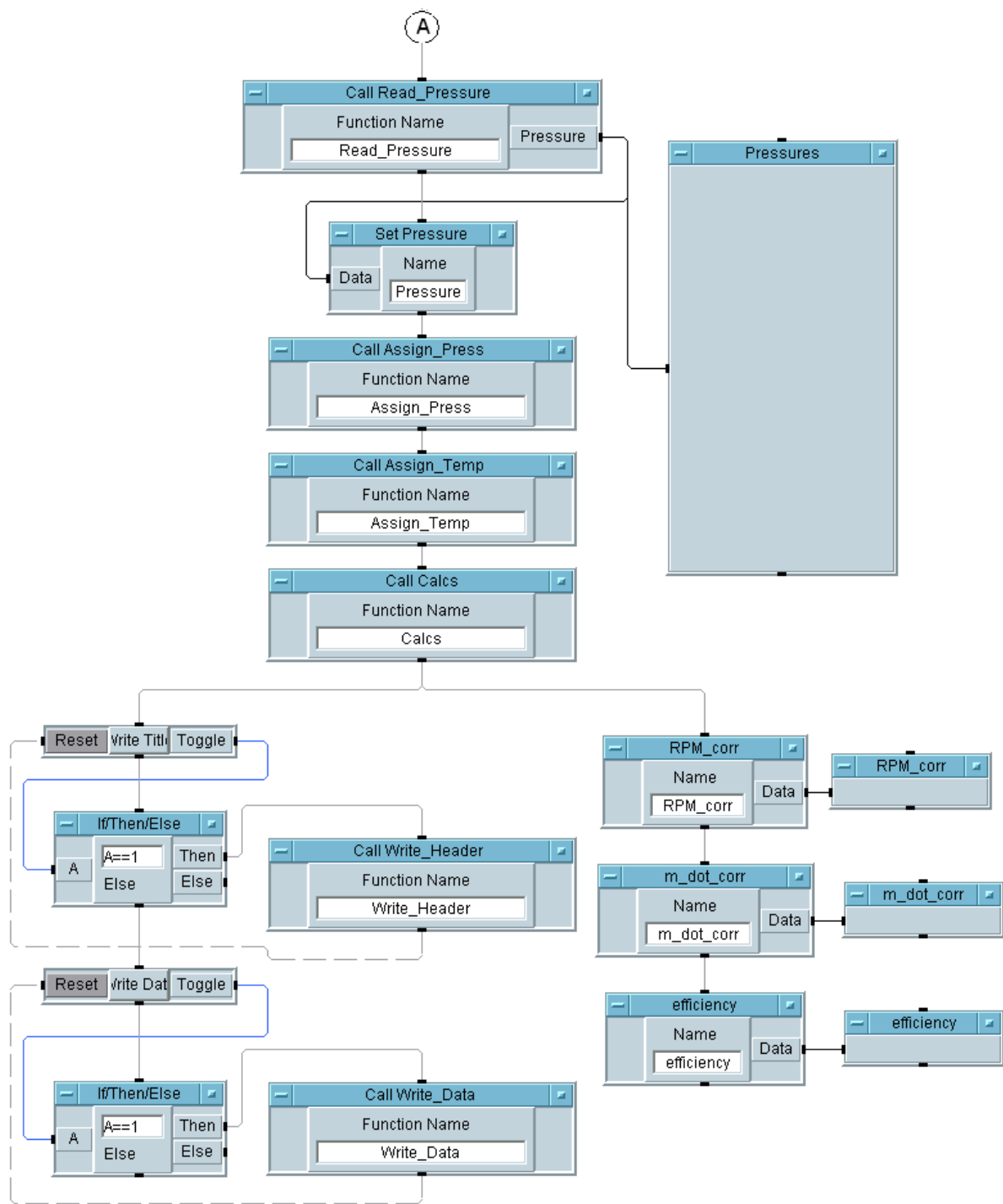
Figure A.02 “MAIN” function, page 2
