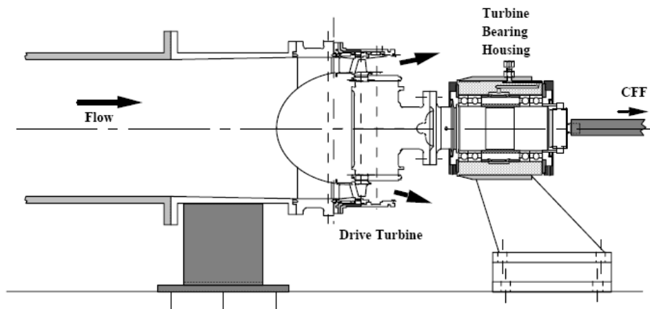
Figure 5. Schematic of Turbine Test Rig. From [8]
