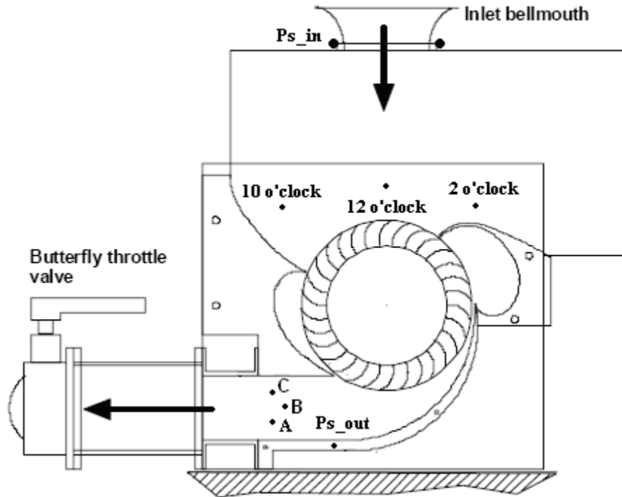
Figure 8. Location of Combo Probes and Static Pressure Taps
