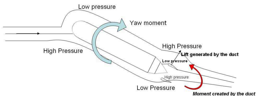
Figure 2.6.16: Pressure distribution along the body of the RPUUV with the duct.
