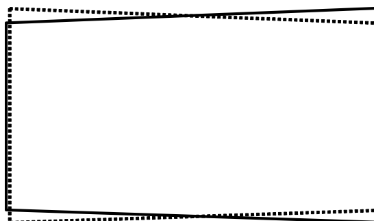
Figure 3.4. If the projectors are positioned side-by-side, the keystoneing of one projected image (solid-line figure) will be opposite that of the other projected image (dashed-line figure), preventing good registration of the two images.
