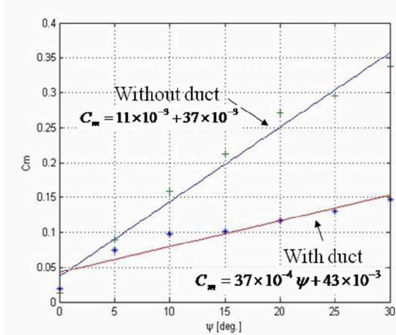
Figure 2.6.14: Yaw moment coefficient as a function of yaw angle \psi at R_2 .
