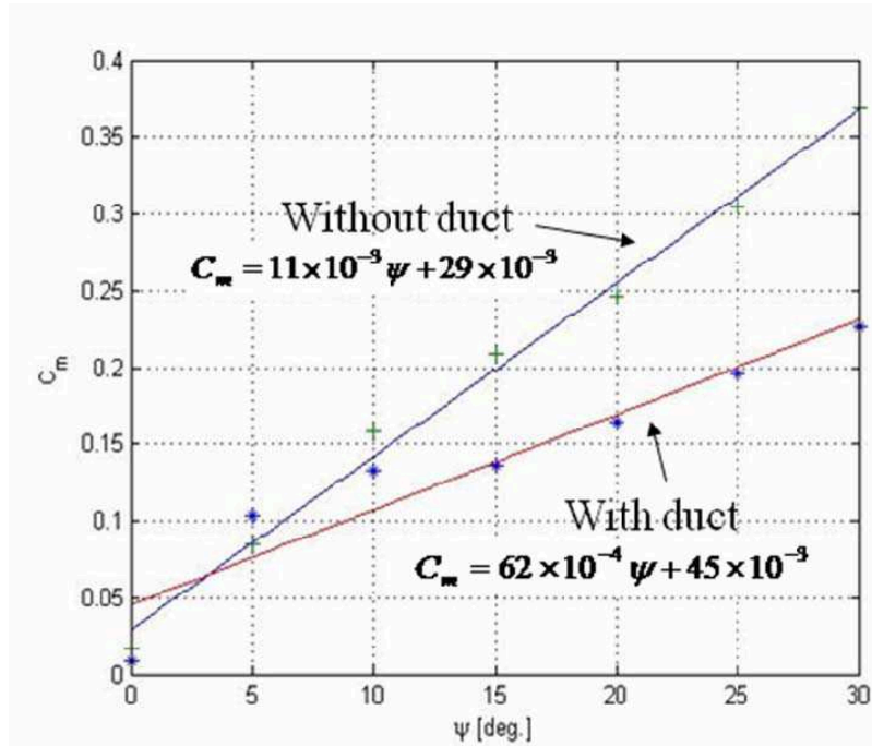
Figure 2.6.13: Yaw moment coefficient as a function of yaw angle \psi at R_1 .
