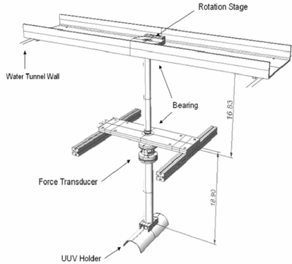
Figure 2.6.6: RPUUV sting design.
