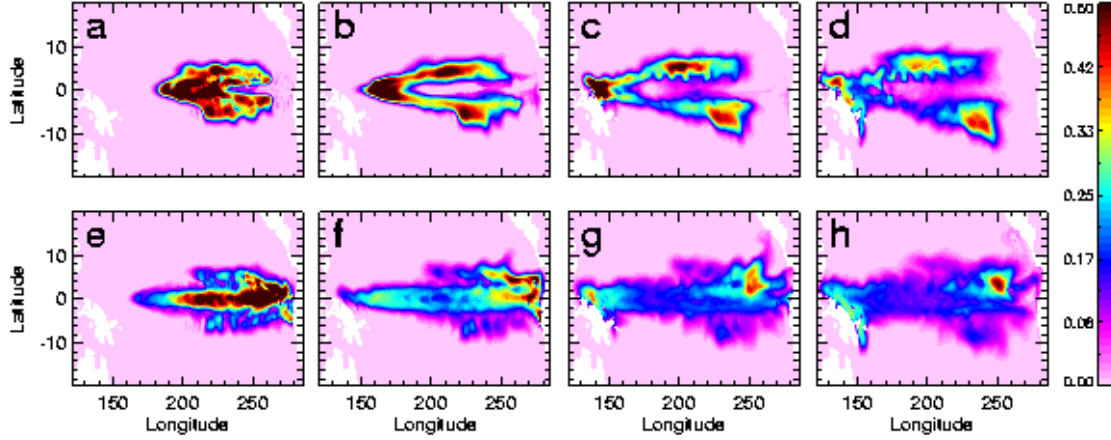
Figure 5: Temporal evolution of vertically integrated adjoint tracer distribution (arbitrary tracer unit) released in the pycnocline ( 24.5 \leq \sigma_\theta \leq 26 \text{ kg m}^{-3} ) of the eastern equatorial Pacific ( 5^\circ\text{S} \sim 5^\circ\text{N} , 150^\circ\text{W} \sim 90^\circ\text{W} ) at the end of 1997 (a, b, c, d) and the end of 1996 (e, f, g, h). The former is an El Niño year and the latter is a non-El Niño year. The panels are, from left to right, -3 (a, e), -6, (b, f), -9 (c, g), and -12 (d, h) months from the end of the respective years.
