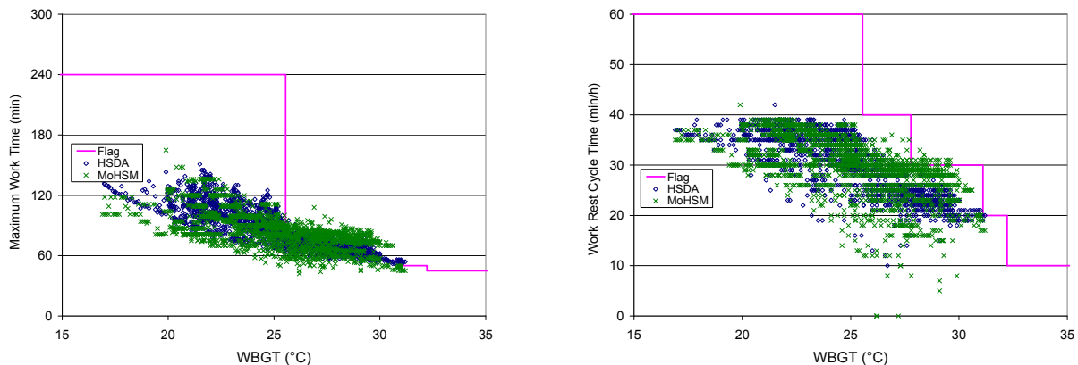
Figure 2c. MXWRK and WRC Guidance for Heavy Work at FTB and GIIB
