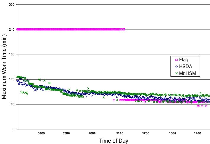
Figure A-1f. Maximum Heavy Work (600 W) Guidance for FTB
