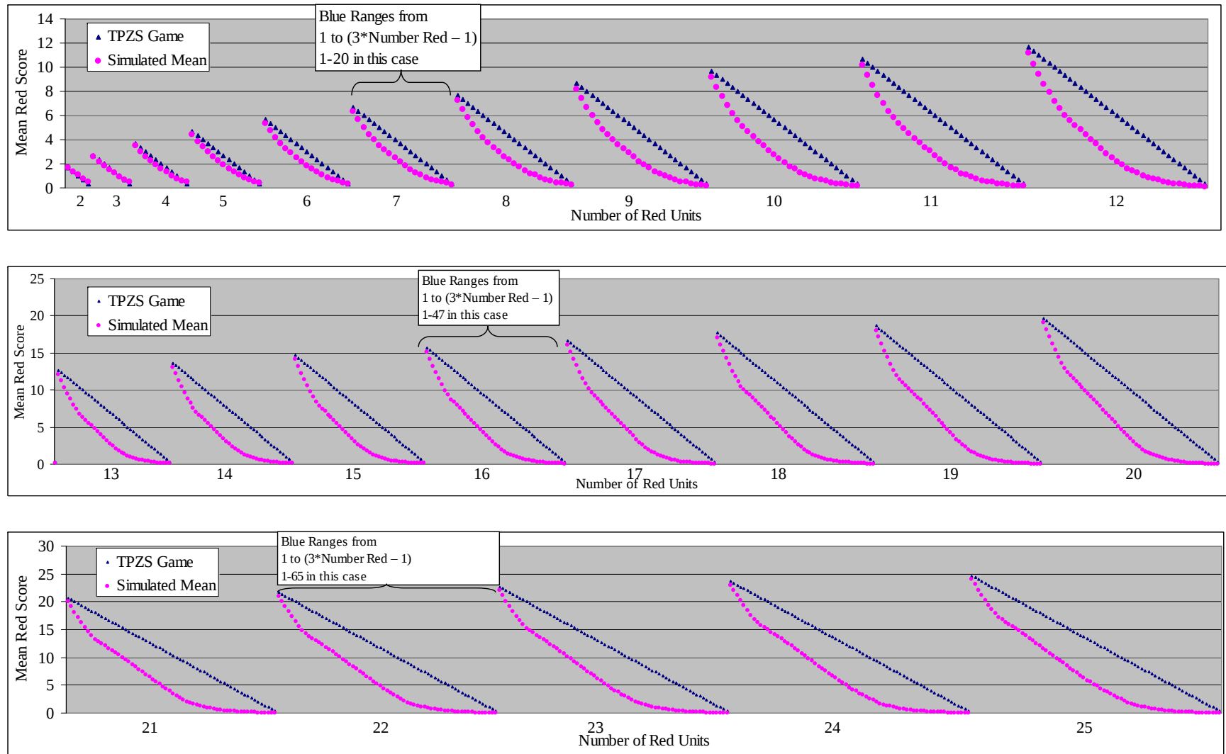
Figure 17. Comparison of Red Scores with Sensors to Red Scores without Sensors
