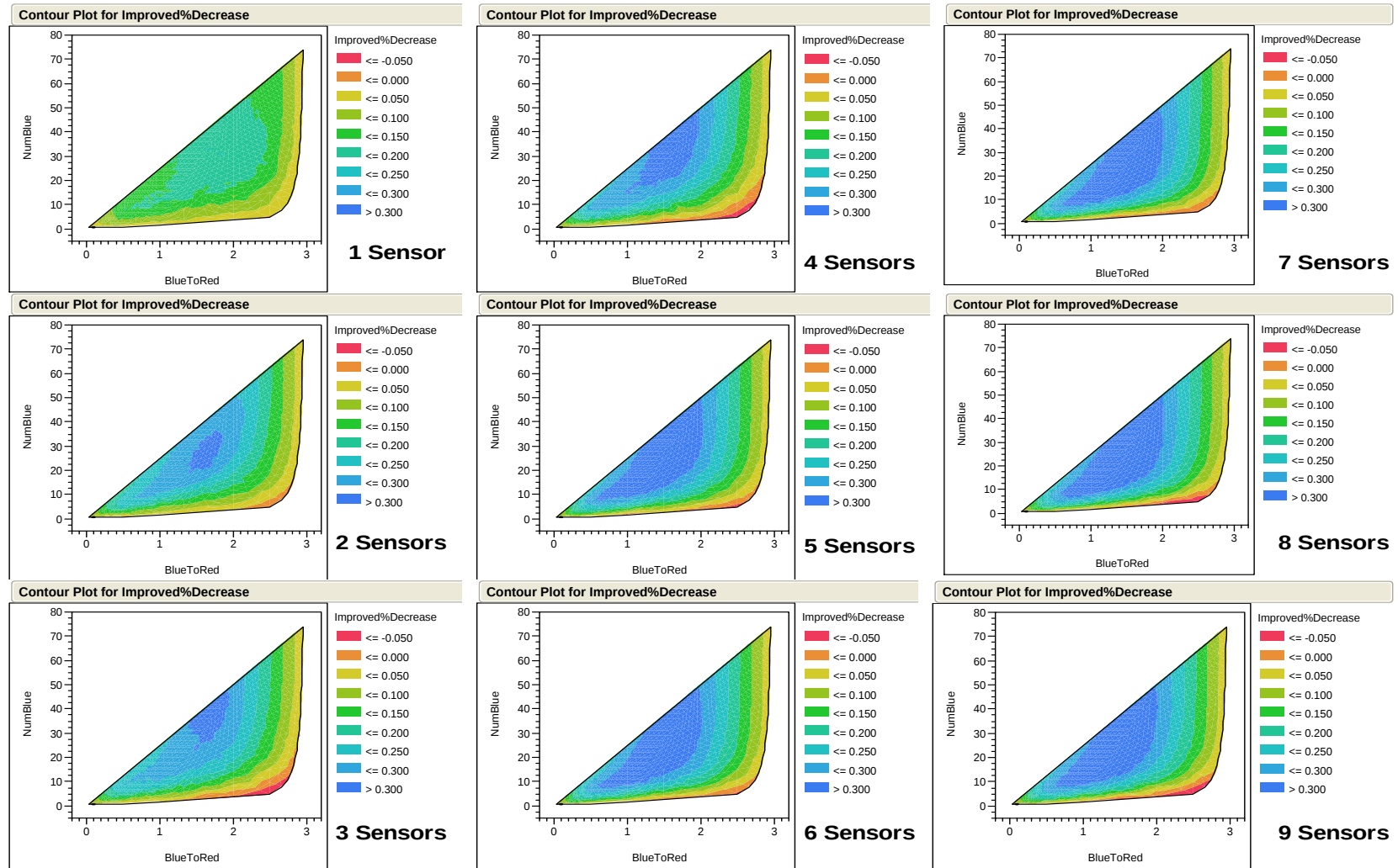
Figure 19. Contour Plots by Sensor for Number of Blue Units vs. Blue to Red Ratio
