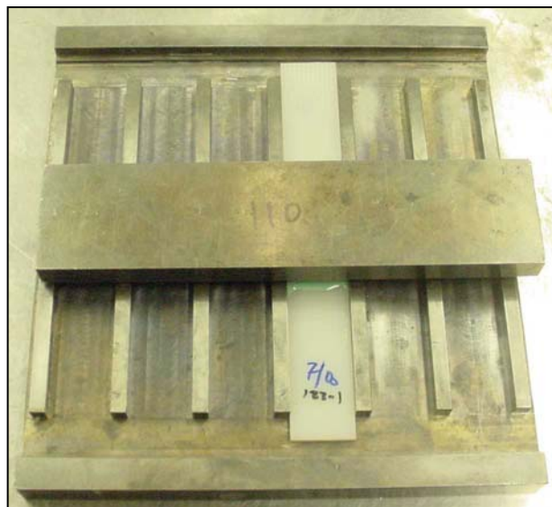
Figure 20. Improved Nylon 6,6 Lap Shear Holding Fixture
