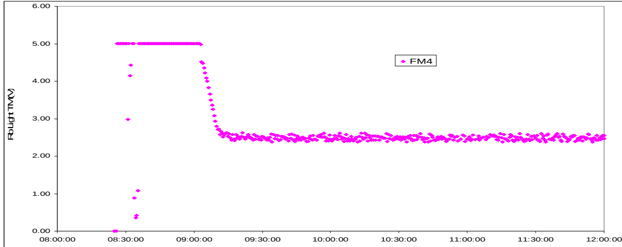
Figure 15. RAFS FM4 Rb light TM during a typical switch-on sequence.
