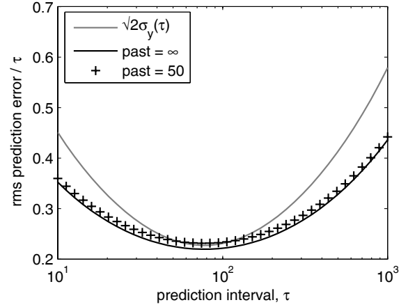
Fig. 2. Normalized rms error of predictors of a sum of white FM and random walk FM.
