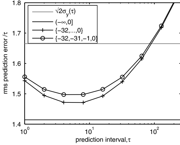
Fig. 4. Normalized rms errors of predictors of flicker FM
