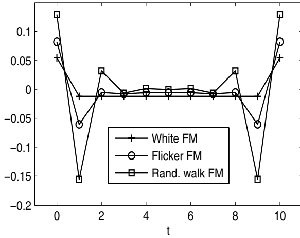
Fig. 5. Regression coefficients for estimating quadratic drift rate in the presence of white FM, flicker FM, or random walk FM.
