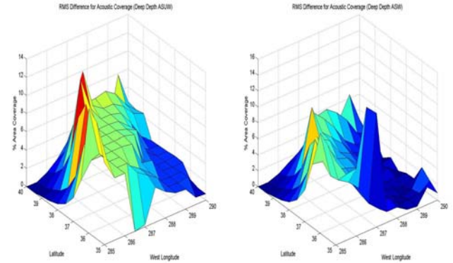
Fig. 13. RMSD for deep depth band coverage: left panel for ASUW scenario and right panel for ASW scenario.
