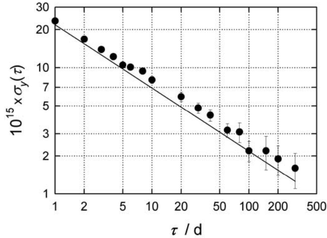
Figure 4. Relative instability of the frequency difference \gamma (CS1 – CS2), recorded between MJD 50800 and MJD 53300, expressed by the non-overlapping Allan standard deviation \sigma_y(\tau) .
