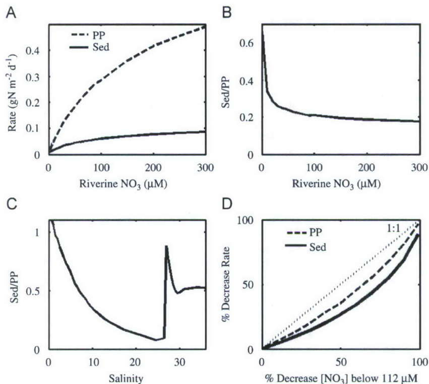
Fig. 7. Effect of variable riverine \text{NO}_3 loading on average rates of (A) primary production (PP) and sedimentation (Sed), and the ratio Sed/PP versus (B) \text{NO}_3 loads and (C) salinity. The example in panel C is for a \text{NO}_3 load of 112 \mu\text{M} (the long-term mean). As well, the relationship between decreasing \text{NO}_3 load and decreases in average primary production and sedimentation are shown (panel D). These decreases were calculated relative to a 112 \mu\text{M} \text{NO}_3 load scenario for which average primary production and sedimentation equaled 0.31 and 0.063 \text{gN m}^{-2} \text{d}^{-1} , respectively. This panel addresses the potential impacts of mandated reductions in \text{NO}_3 loading to the Mississippi River watershed. For example, a 30% decrease in \text{NO}_3 below 112 \mu\text{M} would decrease average PP by 19% and average Sed by 14%. All average values of primary production and sedimentation were calculated for intermediate to high salinities ( >15 ).
