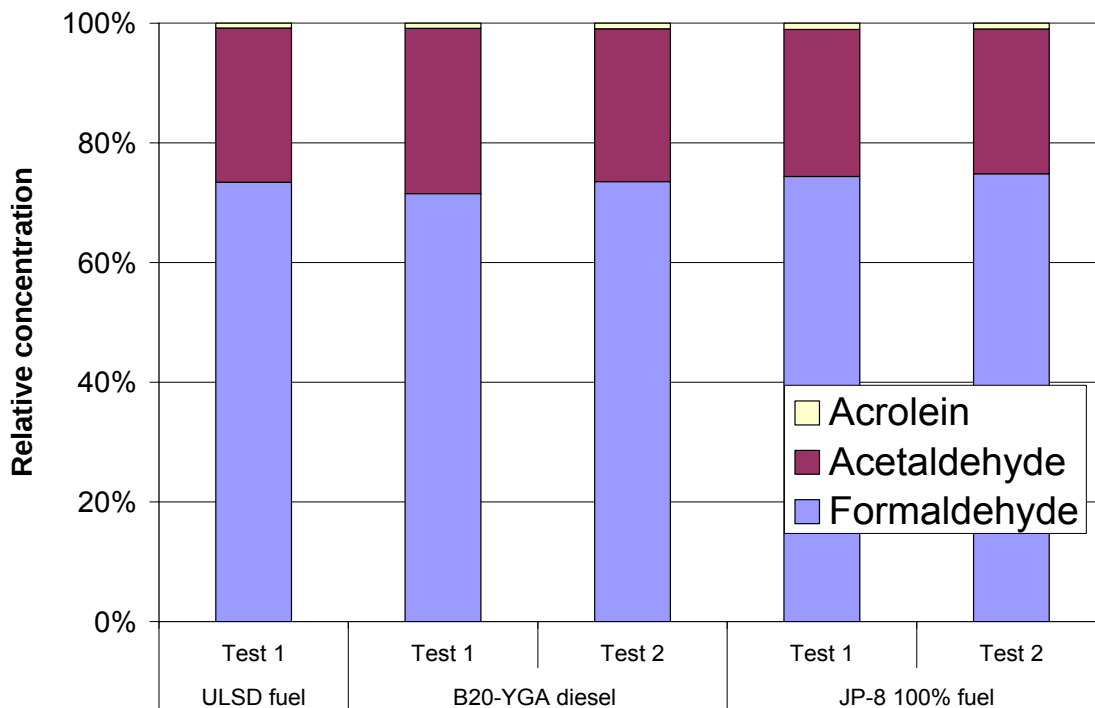
Figure 4.26 Humvee Relative Carbonyl Emissions
