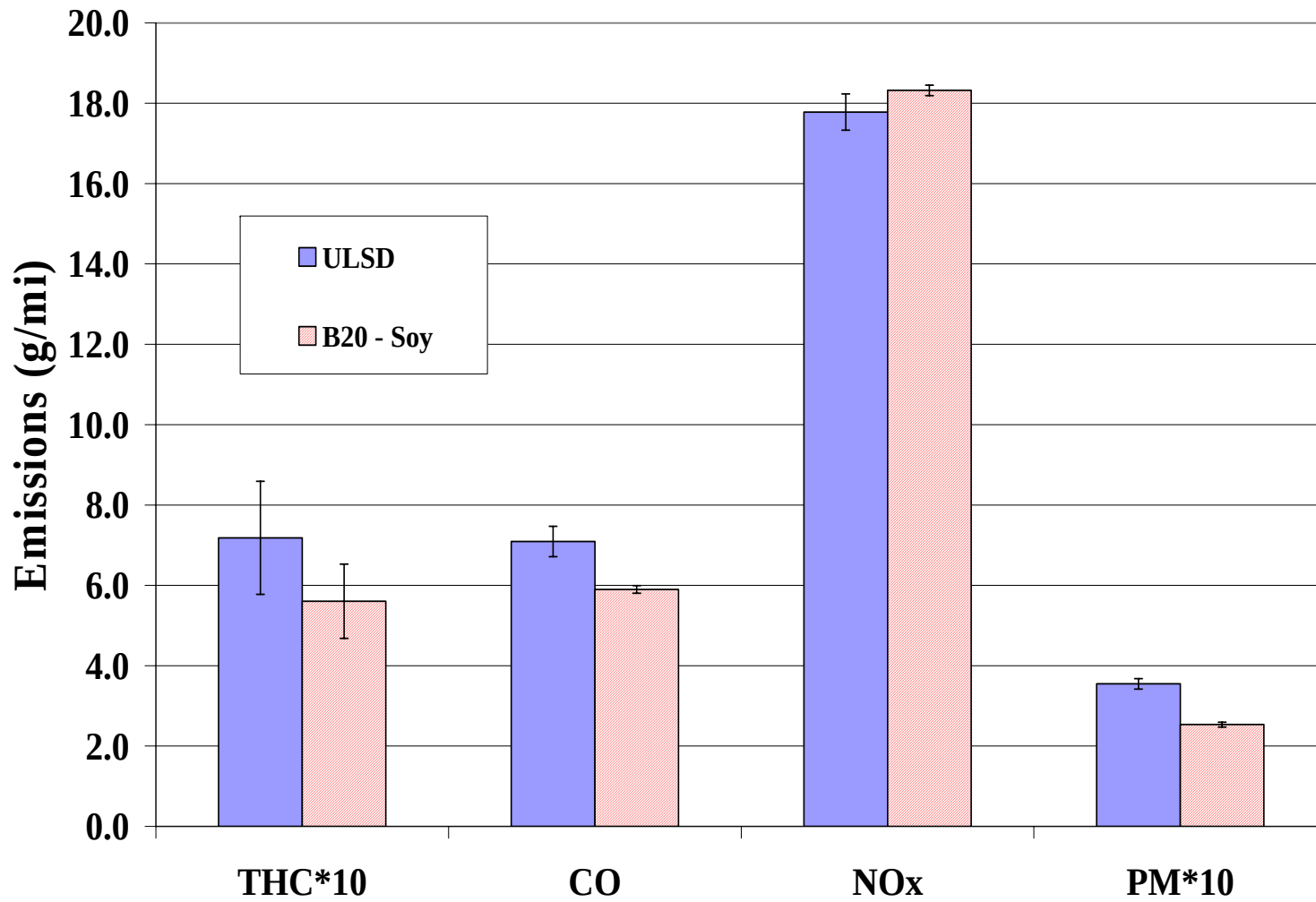
Figure 4.8 UCR-Cheyenne Mountain Cycle Results – Cheyenne Mountain Bus
