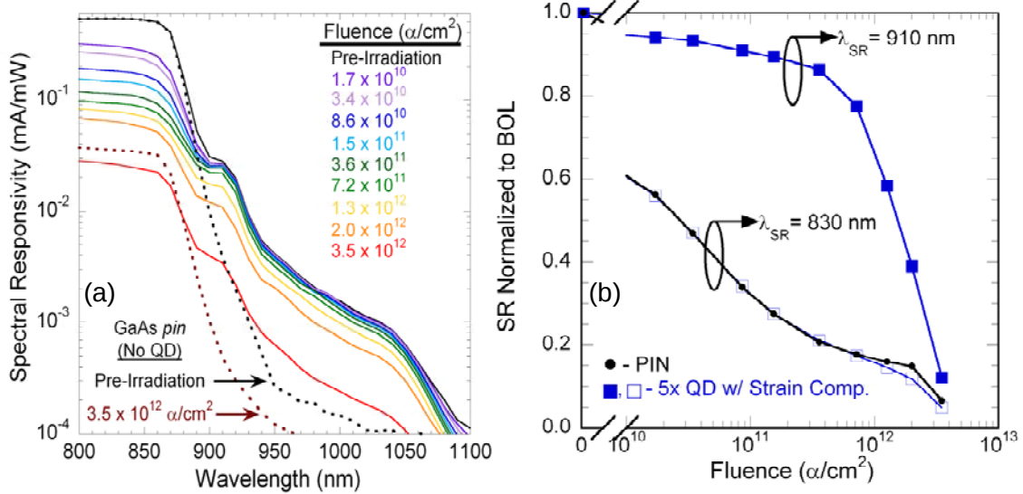
Figure 6. (a) Spectral response of the QDSC at incremental levels of alpha-particle fluence; the pre-irradiation and post 3.5 \times 10^{12} alpha-particle/cm 2 response spectra of the baseline device are overlaid for comparison. (b) The spectral response as a function of fluence measured at 830 nm for both devices and at 910 nm for the QDSC.
