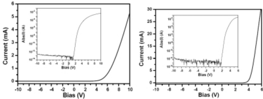
Figure 6. (Left) Current-voltage characteristics of a photodiode on AlN template ( \sim 300 nm p-GaN/ 150 nm i-GaN/ 400 nm n-GaN) in linear and logarithmic scale (inset). The turn-on voltage was \sim 6.2 V, ideality factor was \sim 3.32 , and series resistance was \sim 521 \Omega . (Right) Current-voltage characteristics of a photodiode on GaN template in linear and logarithmic scale (inset). The turn-on voltage was \sim 4.28 V, ideality factor was \sim 2.45 , and series resistance was \sim 39.4 \Omega .
