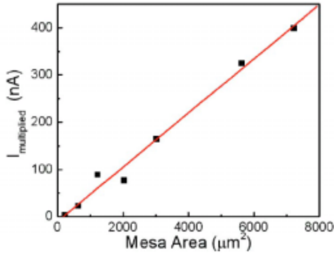
Figure 14. Multiplied current component of the dark current as a function of mesa area.
