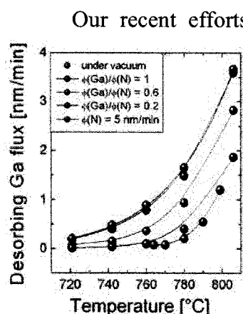
Fig. 1: Reduced Ga desorption (i.e. decomposition rate) with N-rich conditions. (2007).
