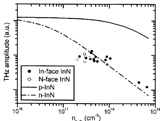
FIG. 3. Terahertz amplitude dependence on bulk carrier density n_{\text{bulk}} for In- (solid circles) and N-face (empty circles) InN samples optically excited with 800 nm femtosecond pulses. Calculated results for p -type and n -type InN are shown with solid and dashed lines, respectively.
