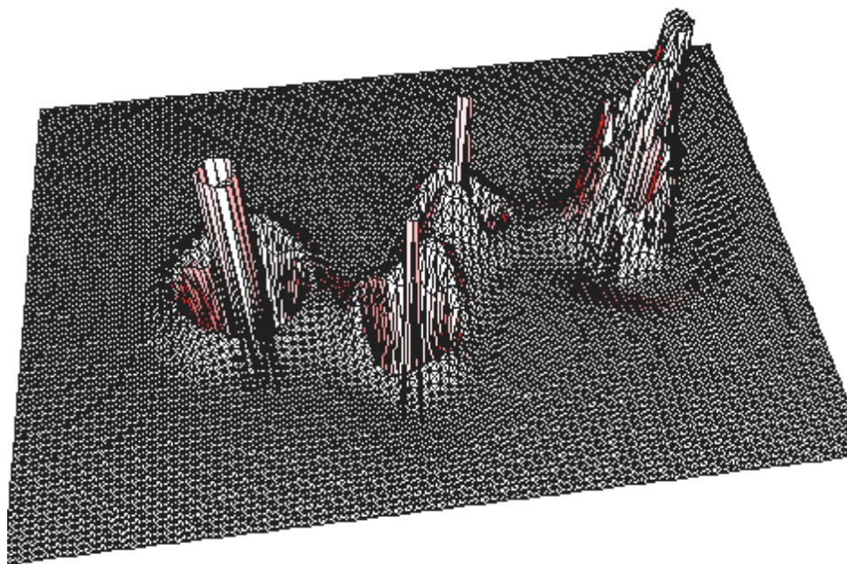
Figure 1. Laplacian of the Electron Density of the Transition State for Thiirane + NH_3
