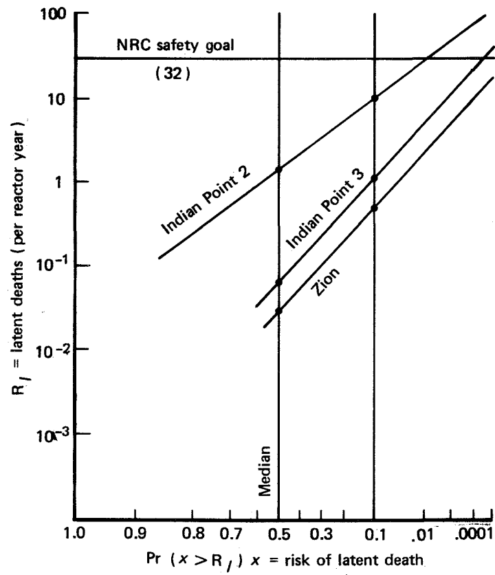
Fig. 7 -- Confidence values: latent deaths, Weibull distribution
