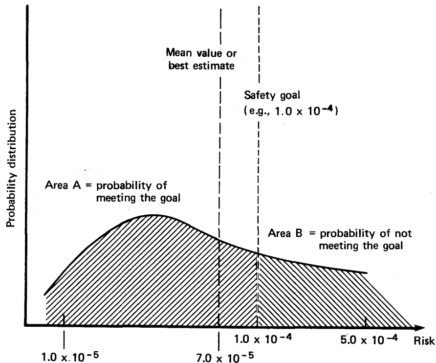
Fig. 1 -- The confidence in risk estimate concept: risk of core melt per reactor year
