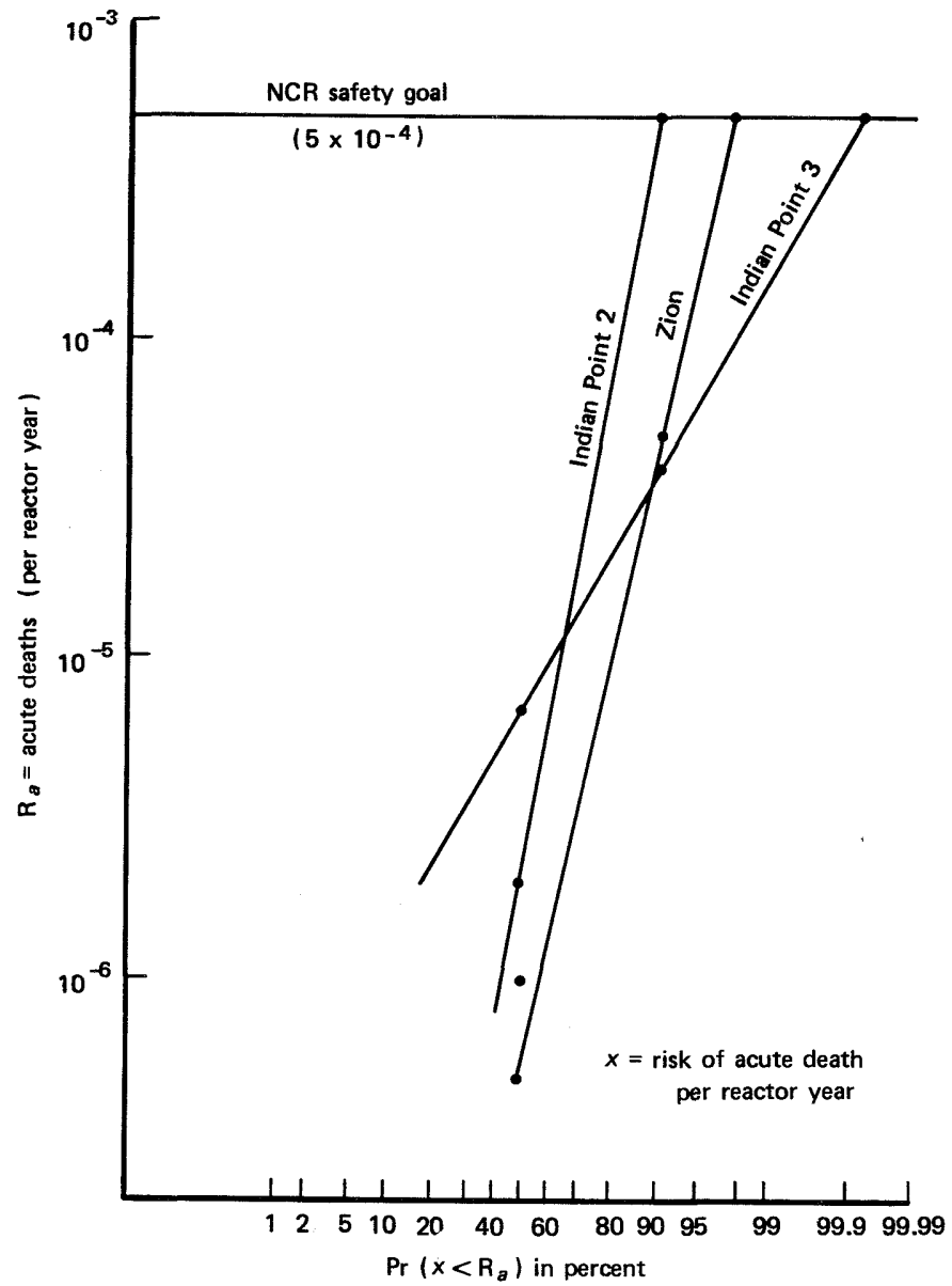
Fig. 3 -- Confidence values: acute deaths, log-normal distribution
