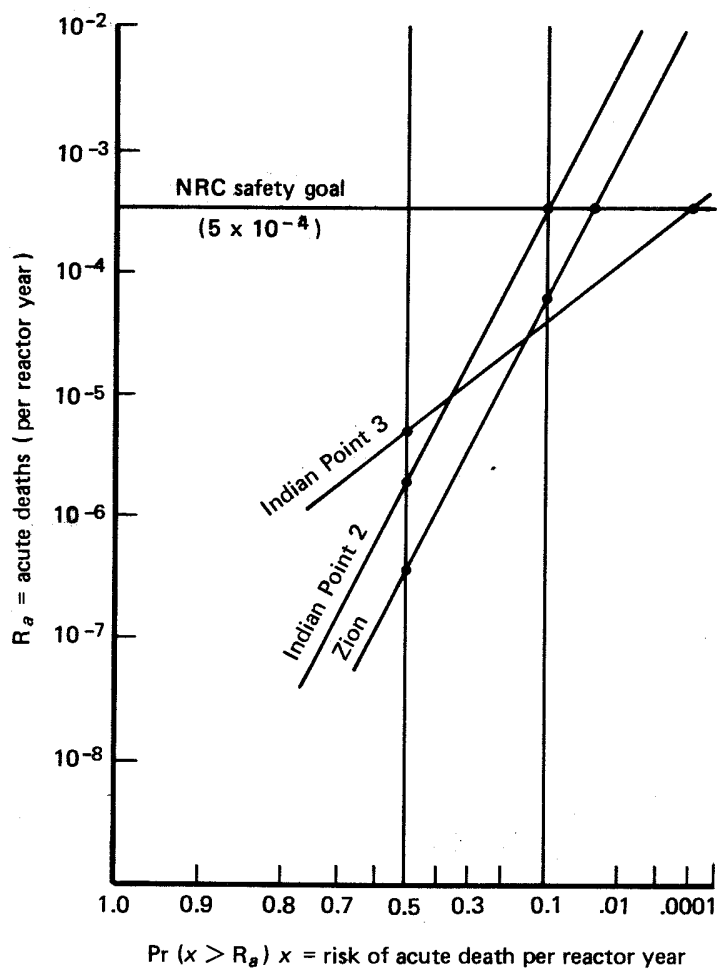
Fig. 6 -- Confidence values: acute deaths, Weibull distribution
