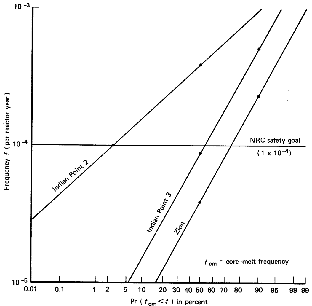
Fig. 2 -- Confidence values: core melt, log-normal distribution
