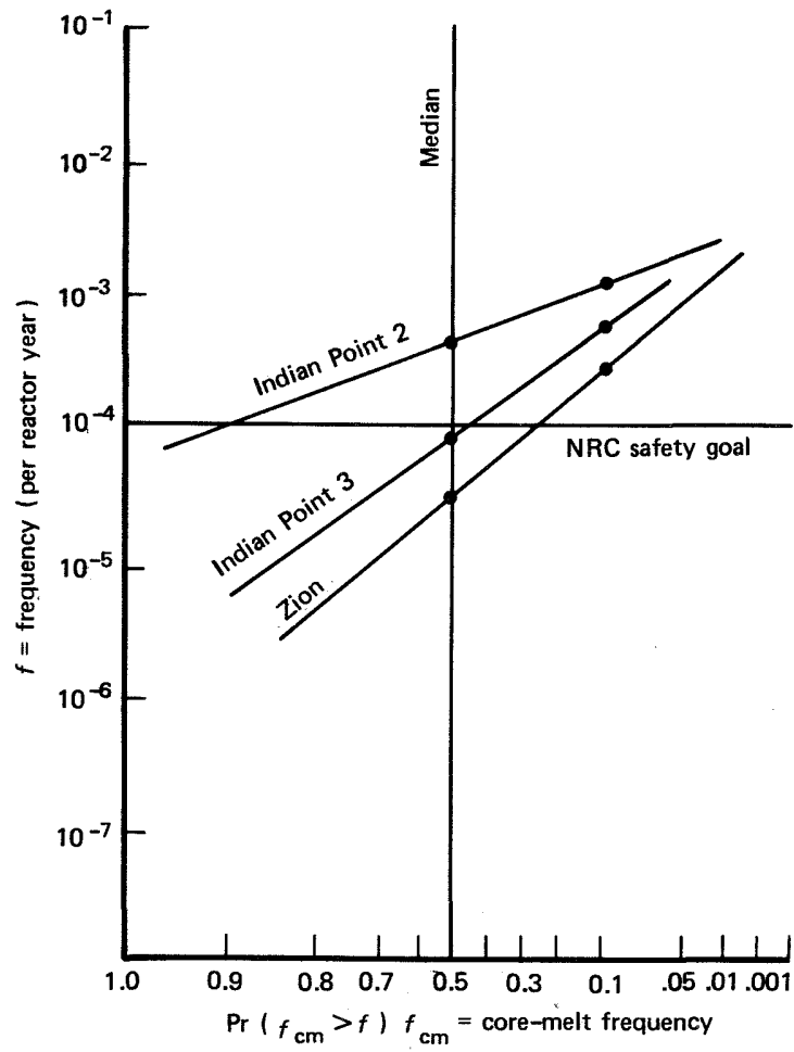
Fig. 5 -- Confidence values: core melt, Weibull distribution
