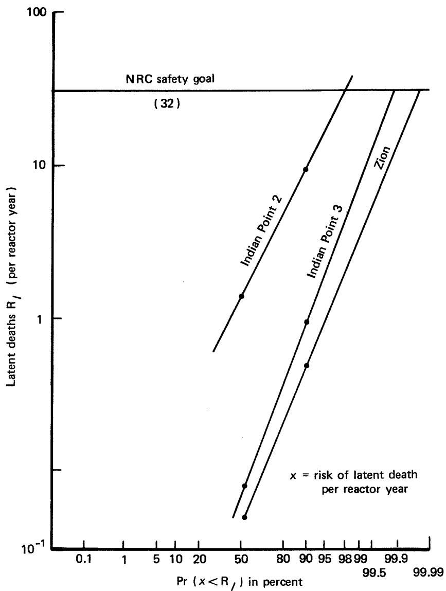
Fig. 4 -- Confidence values: latent deaths, log-normal distribution
