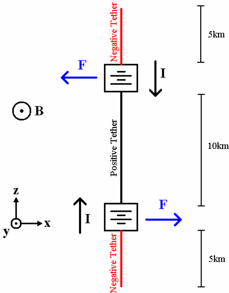
Figure 2-7: Series Tether
