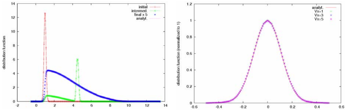
Figure 16. Ions distribution functions along \xi_y = 0 line for different time moments (left) and distribution functions vs \xi_x lines for different \xi_x positions (right).
