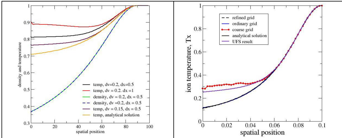
Figure 4. UFS ion density and temperature from (on the left) for different size of velocity and space mesh. Ion temperature from Shoucui's code and UFS (on the right)
