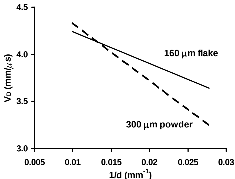
Figure 16. A representation of the results of Maranda et al. [24] showing the effect of particle size upon the detonation performance of 80:10:10 AN/TNT/Al formulations containing micrometric aluminium powder.
