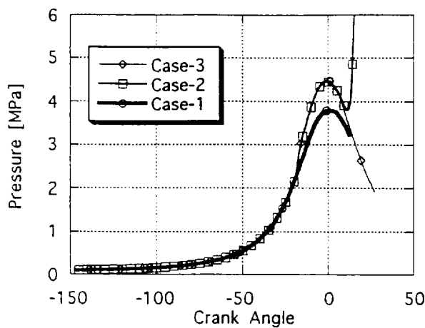
Figure 5 Engine pressure for cases 1,2, and 3.
