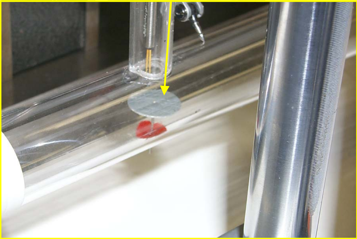
Figure 8. Experimental Setup For Velocity Measurements Through a Prototype TGA 951 Wind Tunnel
