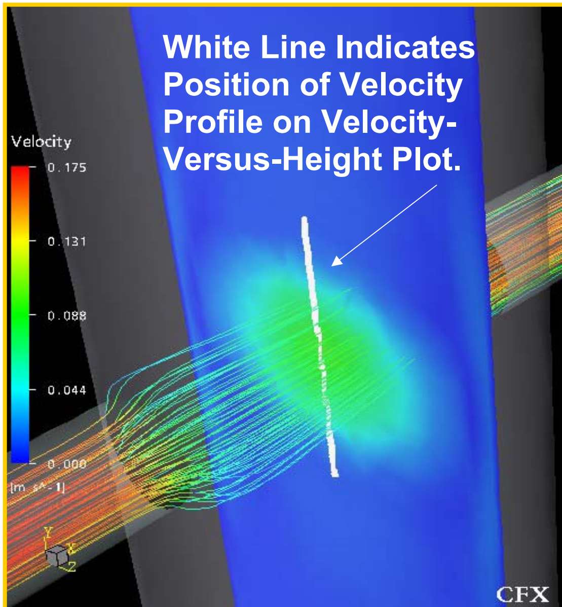
Figure 18. Three-Dimensional Streamlines and Two-Dimensional Plane for the Velocity versus Height Contour Plot
