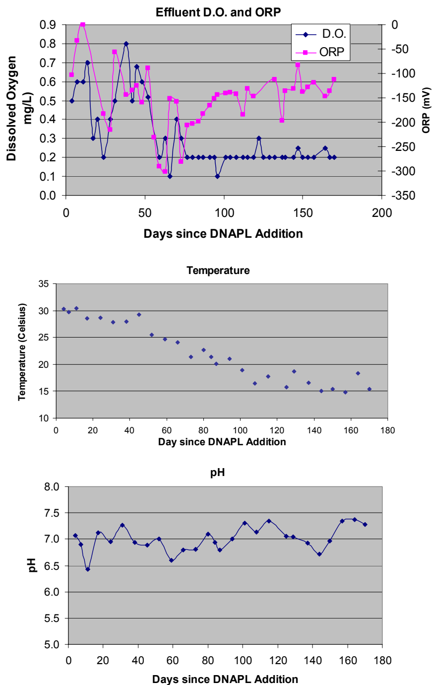
Figure 21. Effluent Monitoring Data for DNAPL Experiment
