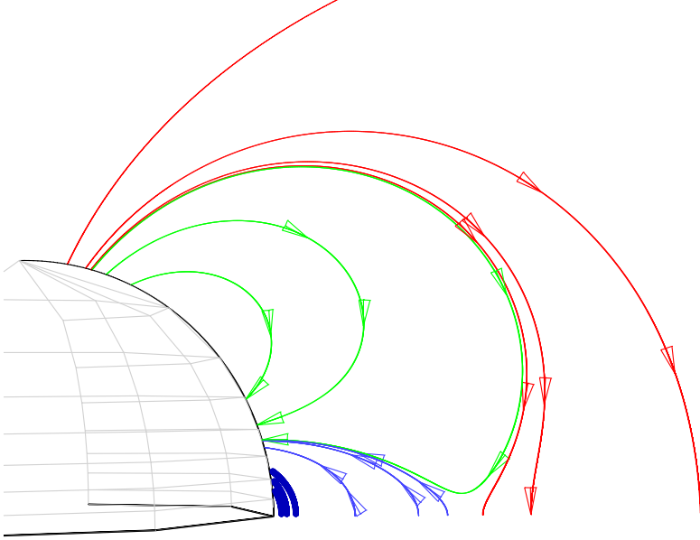
Fig. 1(a) Initial potential magnetic field. The field is symmetric about the axis of rotation and the equator, so only one quadrant is shown. The photospheric boundary surface is indicated by the light grey grid. Magnetic field lines are colored (red, green, or blue) according to their flux system. Two types of blue field lines are indicated, higher-lying light-blue unsheared field and low-lying dark-blue field which is sheared later in the simulation.
