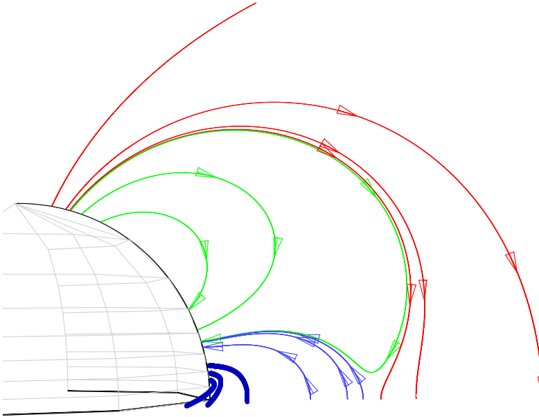
Fig. 4(b) As above, but for a shear of \pi/4 .
