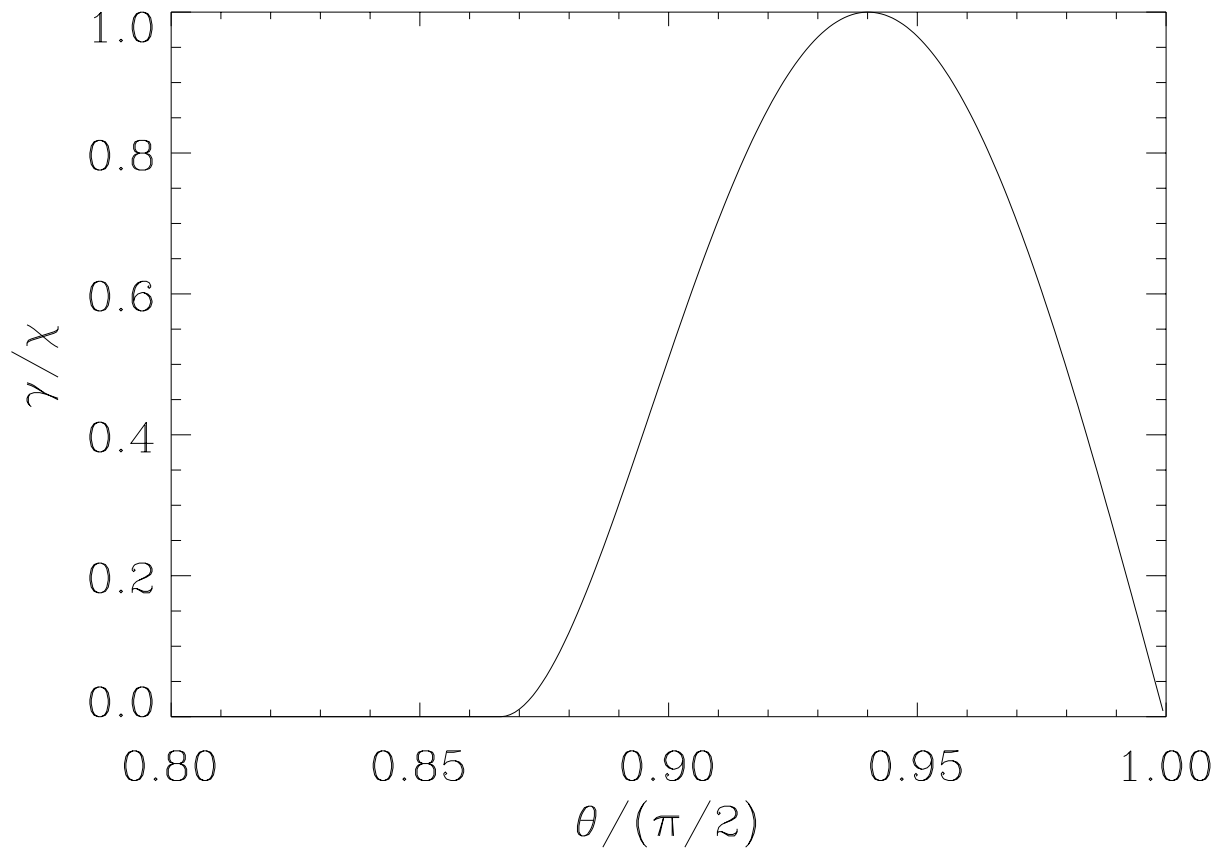
Fig. 2. The normalized shear profile as a function of colatitude.
