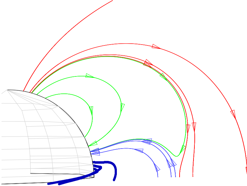
Fig. 4(c) As above, but for a shear of 3\pi/8 .
