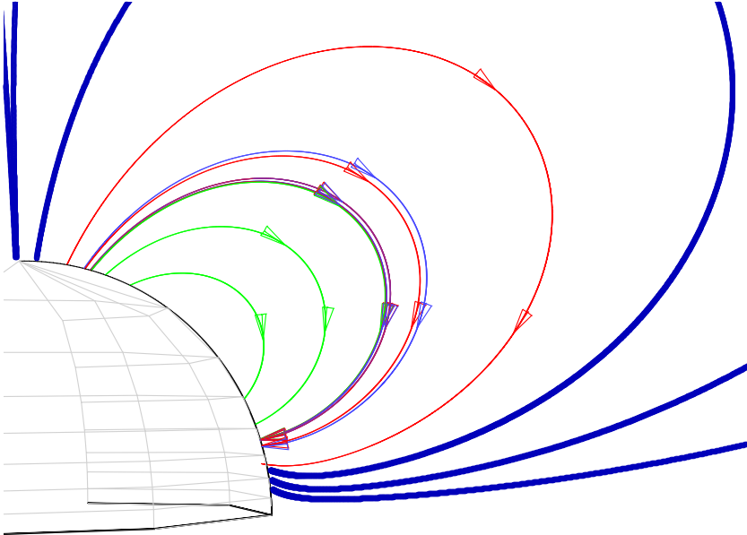
Fig. 1(d) As above, but for a shear of \pi/2 .
