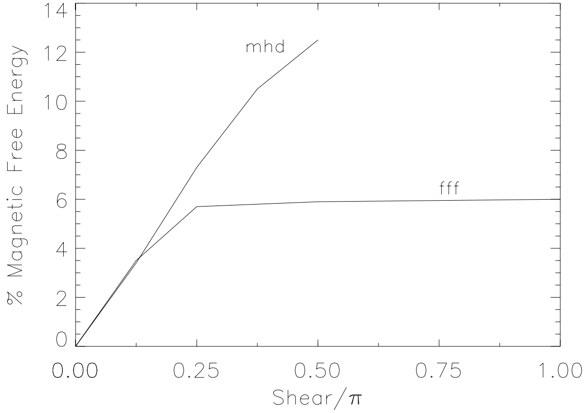
Fig. 3. The magnetic free energy as a function of shear for the force-free field solution (lower curve) and the MHD solution (upper curve). The shear is in units of \pi and the free energy is expressed as percentage of the initial, potential field energy.
