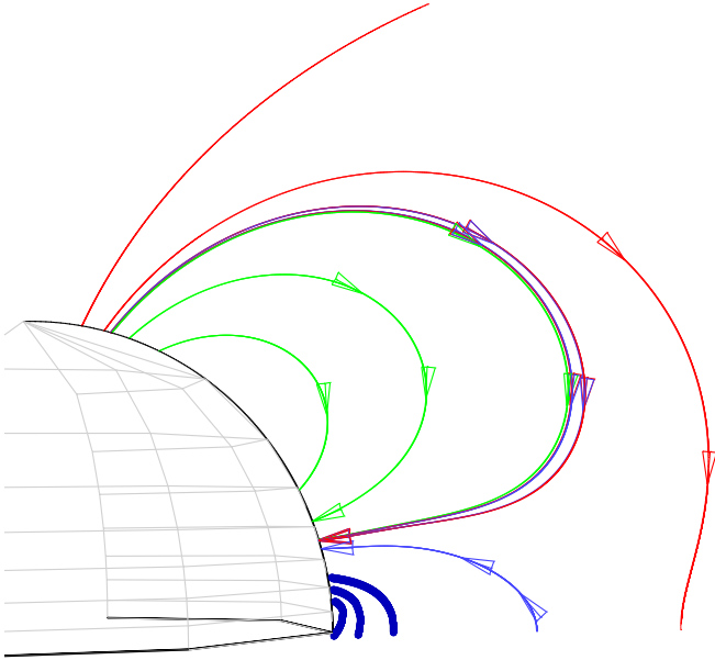
Fig. 1(b) The force-free field after a shear of \pi/8 . The field lines shown correspond to those in 1a. They are traced from the same footpoint position on the photosphere as in 1a.
