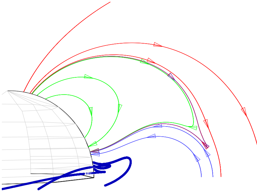
Fig. 4(d) As above, but for a shear of \pi/2 .
