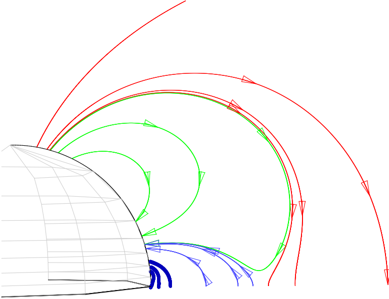
Fig. 4(a) The MHD solution after a shear of \pi/8 . The field lines shown are the same as those in Figure 1.
