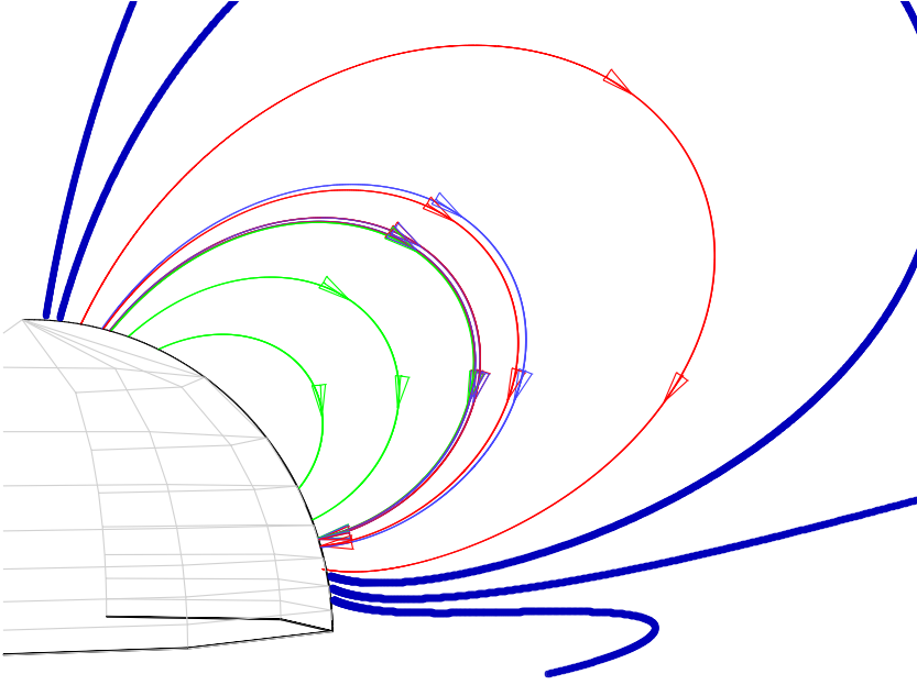
Fig. 1(c) As above, but for a shear of 3\pi/8 .
