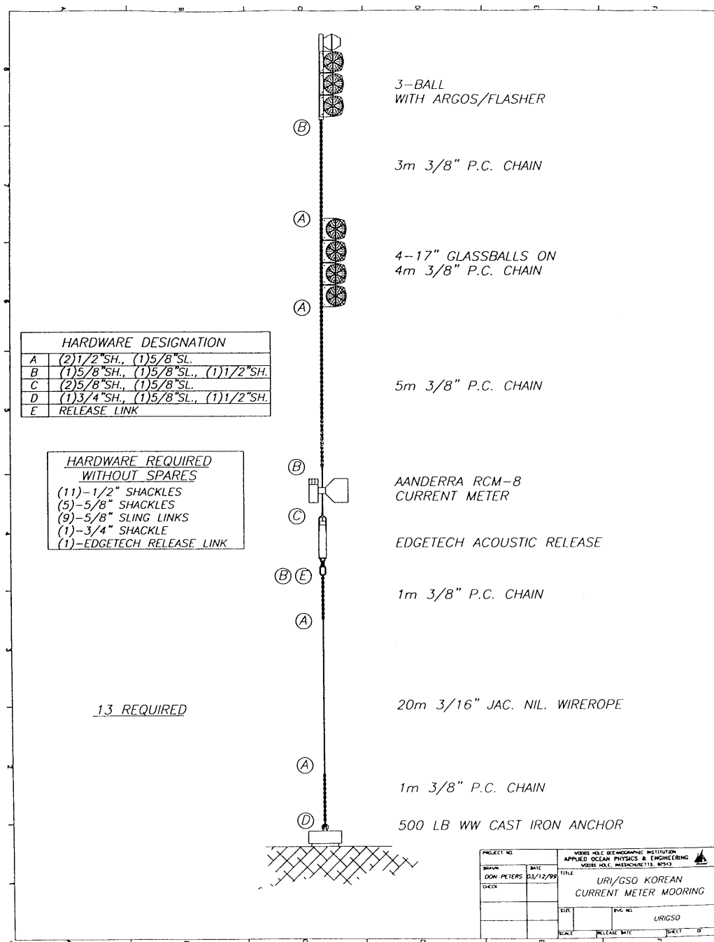
Figure 2: Schematic of the mooring designs of the Aanderra current meter. Glass balls and 500 lb anchor were used to hold the mooring line taut.
