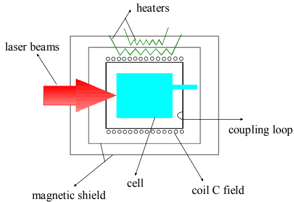
Figure 3. Microwave cavity.
