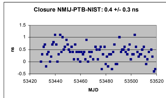
Figure 7. CV transfer across three stations back to the first. Non-zero values indicate error levels.
