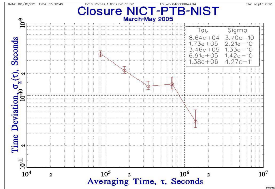
Figure 9. A CV closure using a different set of stations. There is evidence of a systematic change in the residuals.
